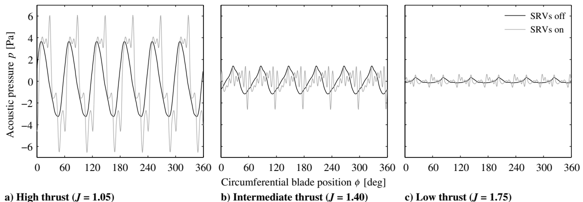
Fig. 19 Acoustic-pressure waveforms at \theta_e = 90^\circ , \phi = 90^\circ .
