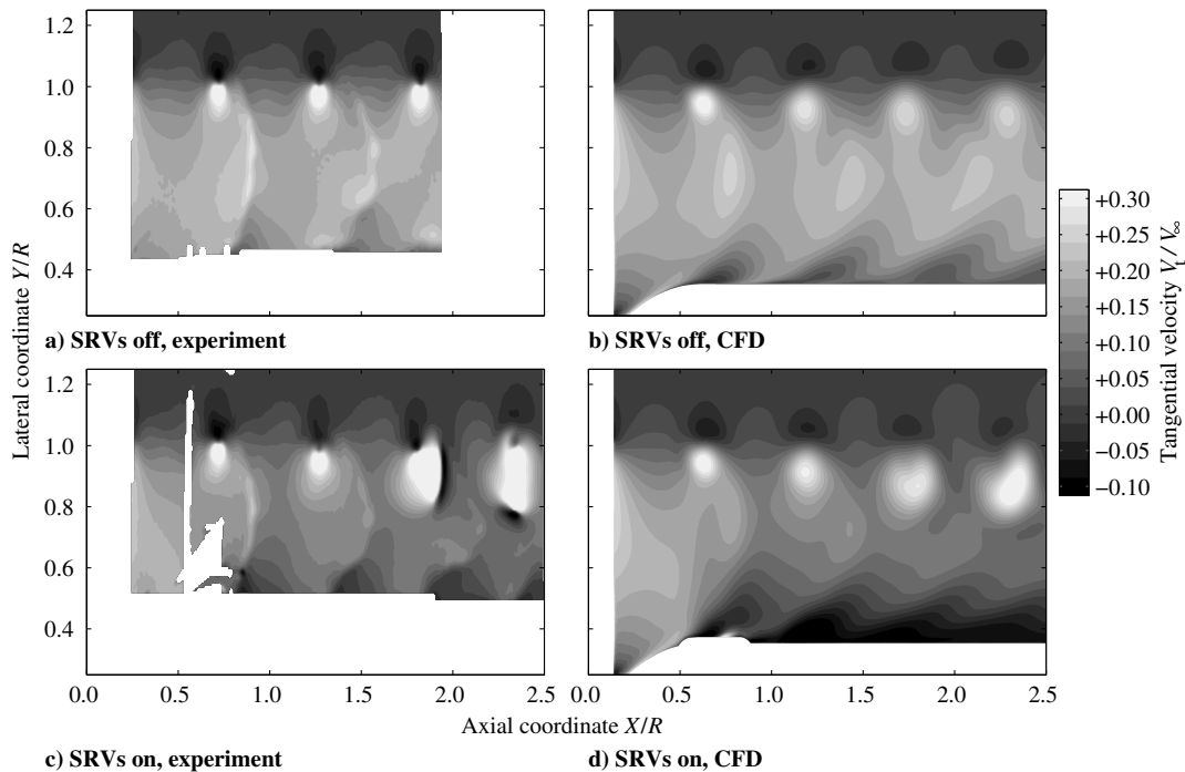
Fig. 9 Phase-locked tangential velocity in the propeller slipstream at Z/R = 0.03 , J = 1.40 .
