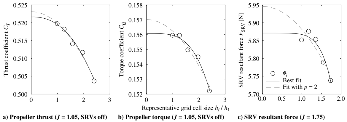
Fig. 8 Grid convergence for a–b) the isolated propeller and c) the propeller with SRVs.
