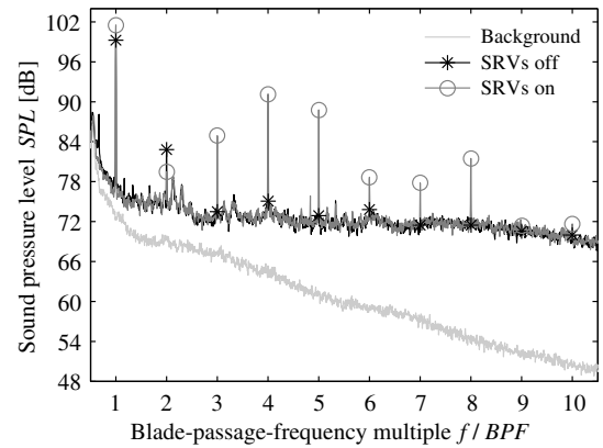
Fig. 20 Sound spectrum at J = 1.05 , \theta_e = 90^\circ , \phi = 90^\circ .
