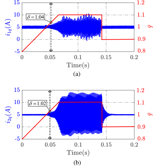
Fig. 10. Experimental results: the critical damping constant \delta testing.
