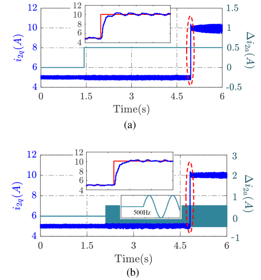
Fig. 11. Experimental results: current control performance with stepping offset disturbance and sinusoidal wave disturbance in i_{2a} .
