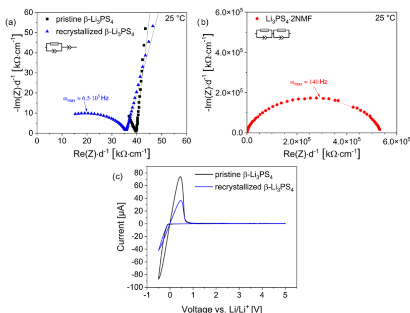
Figure 7. Nyquist plots of pristine and recrystallized \beta - \text{Li}_3\text{PS}_4 (a) and \text{Li}_3\text{PS}_4 \cdot 2\text{NMF} (b) measured at 25 °C with corresponding fits. Cyclic voltammograms of the \text{Li}||\beta\text{-Li}_3\text{PS}_4||\text{stainless steel} cells containing pristine and recrystallized \beta - \text{Li}_3\text{PS}_4 (scan rate: 5 \text{mV s}^{-1} ) (c).
