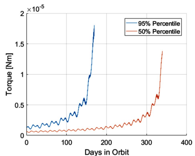
(b) Aerodynamic Torque
