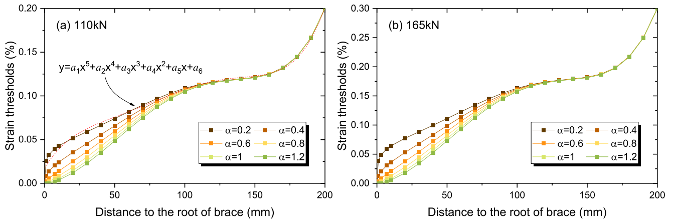
Fig. 16. Strain thresholds in function of crack length on the brace and chord (a) 110kN with considering the interaction; (b) 165kN with considering the interaction.
