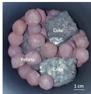
Fig. 8.4 Photograph of the sample bed from the crucible top, before experiment (pellets 10-13 mm and coke 20-25 mm).
