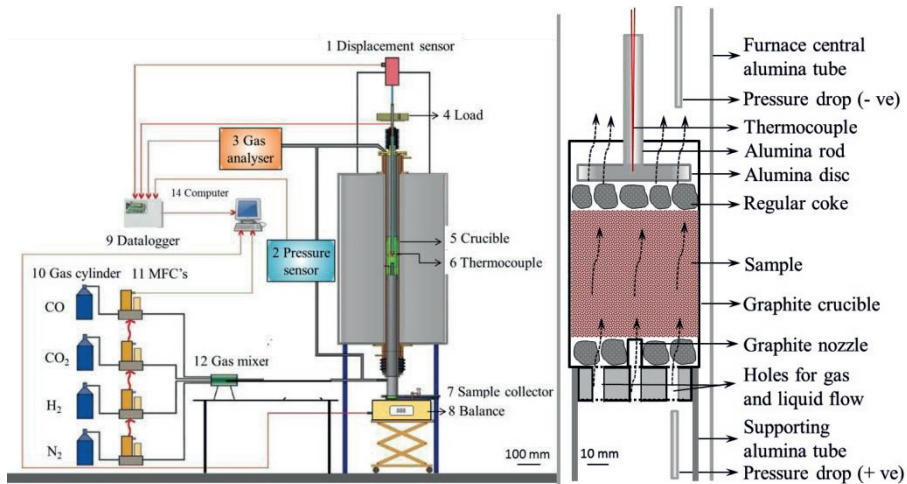
Fig. 3.1 Schematic of Reduction Softening and Melting (RSM) apparatus [3-4].
