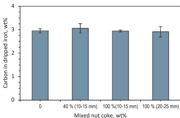
Fig. 8.13 Effect of nut coke addition on the carbon in dripped iron.
