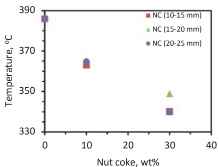
(e). Softening melting temperature range ( T_d - T_I )
