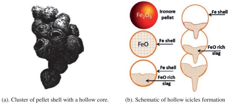
Fig. 4.11 Hollow icicles formation in the cohesive zone, adapted from Gudenau et al. [14].
