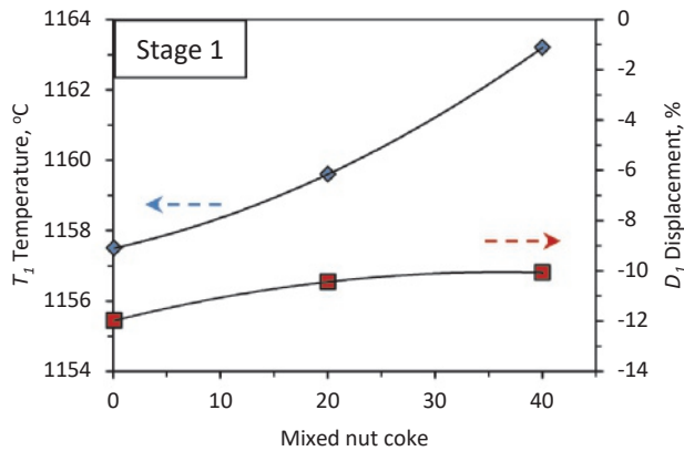
Fig. 7.12 Effect of nut coke addition on the first stage of bed characteristics temperature ( T_I ) and contraction ( D_I ).
