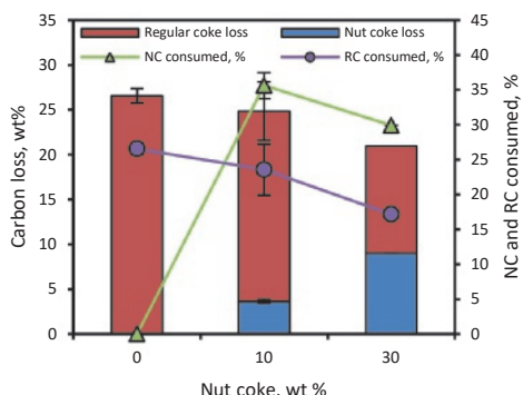
(b). Coke utilisation for pellet bed mixed with 15-20 mm nut coke
