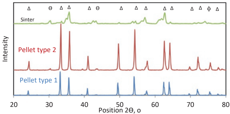
Fig. 3.6 X-ray diffraction (XRD) pattern of ferrous raw materials (Δ- Hematite, φ-Magnetite, Θ- Magnesioferrite).
