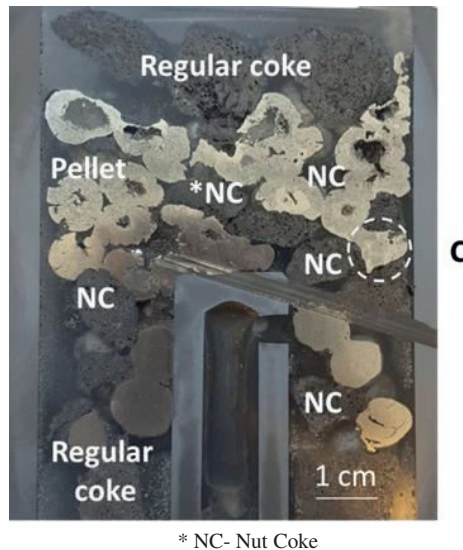
Fig. 6.7 Sample bed with nut coke (40 wt%) quenched at 1450 °C.
