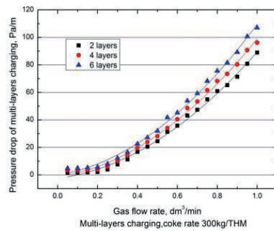
Fig. 2.4 Effect of layers on the pressure drop across the packed bed [13].
