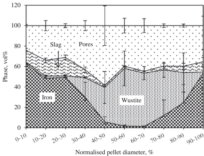
(b). Pellet with mixed (20 wt%) nut coke
