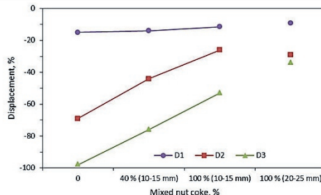
(c) Bed characteristics displacement
