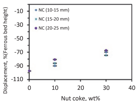
(e). Third stage bed displacement, D_3
