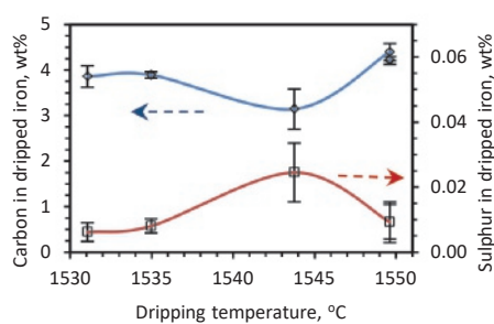
(c). Carbon and sulphur content in the dripped metal
