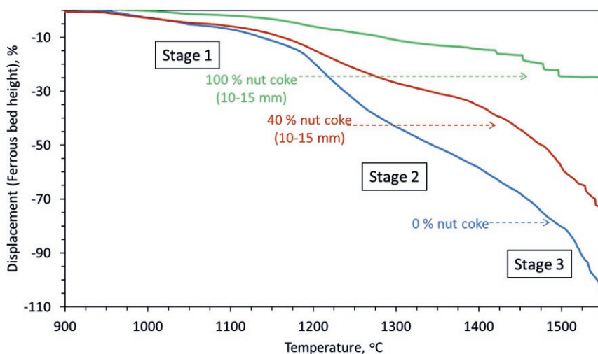
Fig. 8.14 Effect of nut coke addition on bed contraction characteristics of ferrous burden (pellet and sinter mixture).
