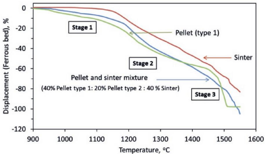
Fig. 7.8 Bed contraction profile for ferrous raw materials.
