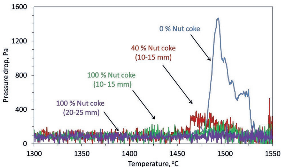
Fig. 8.7 Effect of nut coke addition on pressure drop profile (gas permeability).
