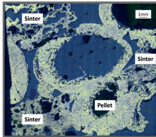
Fig. 7.24 Selected section (region A) from the ferrous bed quenched at 1505 °C without nut coke (Fig. 7.23).
