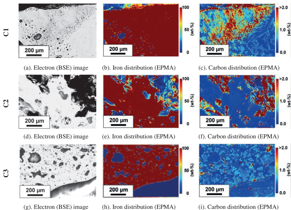
Fig. 6.9 EPMA area scan at location C1, C2 and C3 from Figure 6.8.
