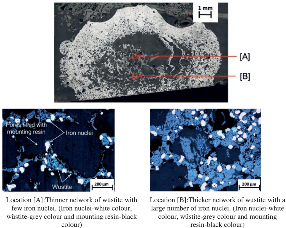
Fig. 4.10 Reflected light microscopy of the pellet quenched from 1400 °C with 20 wt% mixed nut coke.
