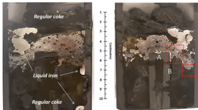
Fig. 7.4 Quenched iron ore sinter bed at 1550 °C.
