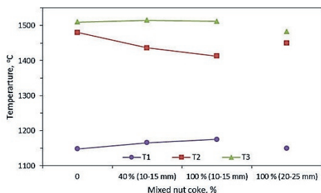
(b) Bed characteristics temperature
