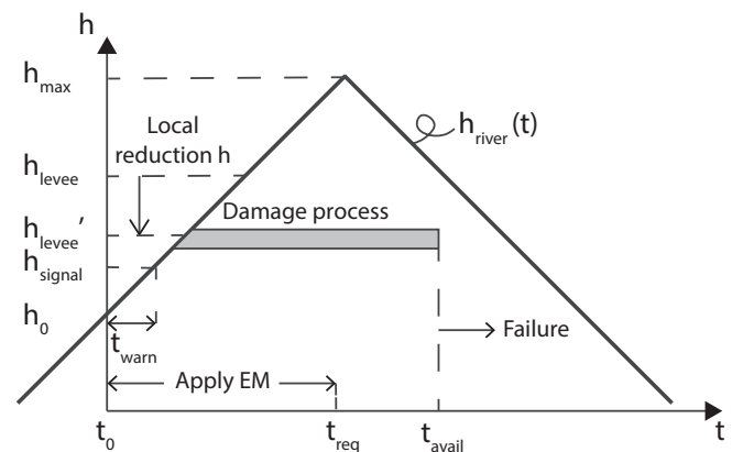
FIGURE 2 | Flood water wave with time required ( t_{req} ) to place an emergency measure (EM) and time available ( t_{avail} ), for scenario with local reduction crest level (from h_{levee} to h_{levee}' ). The thick solid line symbolizes an arbitrary high water wave ( h_{river}(t) ), with a maximum water level h_{max} . The signal water level h_{signal} is the water level at a certain agreed threshold level. The time available between issuing a state of emergency and exceeding the water level threshold is equal to t_{warn} .
