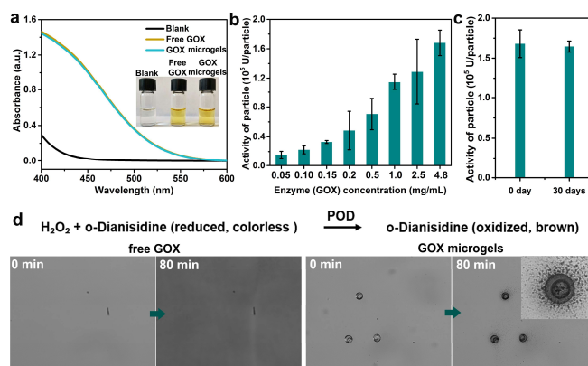
Figure 2. Local generation of H 2 O 2 in the dual-functionalized crescent microgels. a , Absorbance spectra and color change (insert) of the solution without and with free GOX and dual-functionalized microgels in the gluconic acid-specific assay. 10 \mu g/mL free GOX, ~200 particles, 100 mM glucose, 100 mM hydroxylamine and 16 mM Fe 3+ were used in this assay. b , Catalytic activity of the dual-functionalized microgels encapsulated with different concentrations of GOX. c , Stability of GOX in the dual-functionalized microgels after 30 days in PBS buffer solution. d , Visualization of the generation and distribution of H 2 O 2 in the solution with free GOX (left) and dual-functionalized microgels (right, GOX=0.2 mg/mL) through oxidation reaction of o -dianisidine. These results are shown as the mean \pm s.d. of three independent experiments, with ~200 particles for each experiment. Scale bar 200 \mu m.
