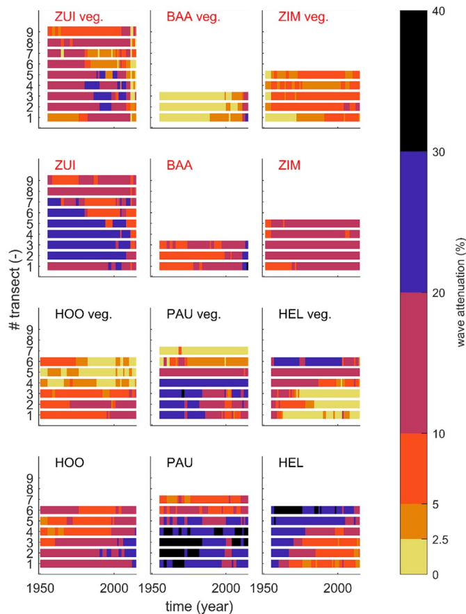
Fig. 7. Wave attenuation (i.e. % of incoming wave; indicated by colors) under design conditions (i.e. extreme event statistically occurring once every 10,000 years) for both the vegetated part of the foreshore (panels with “veg.” behind location name) and the total foreshore. The time is indicated at the horizontal axis, whereas the different transects are presented at the vertical axis. Abbreviations indicate locations as indicated in Fig. 1; red letters highlight exposed sites, while black letters highlight sheltered sites from the prevailing wind direction. (For interpretation of the references to color in this figure legend, the reader is referred to the Web version of this article.)
