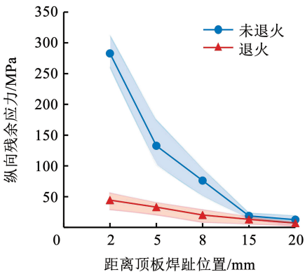
图 10 实测纵向残余应力分布 Fig. 10 Measured distribution of longitudinal residual stress
