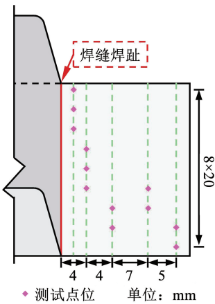
图 9 盲孔法测点布置 Fig. 9 Monitoring point arrangement of hole drill method
