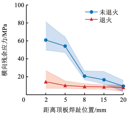
图 11 实测横向残余应力分布 Fig. 11 Measured distribution of transverse residual stress
