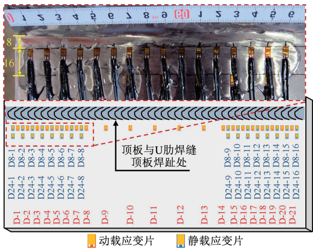
图 8 应变片布置 Fig. 8 Arrangement of strain gauge
