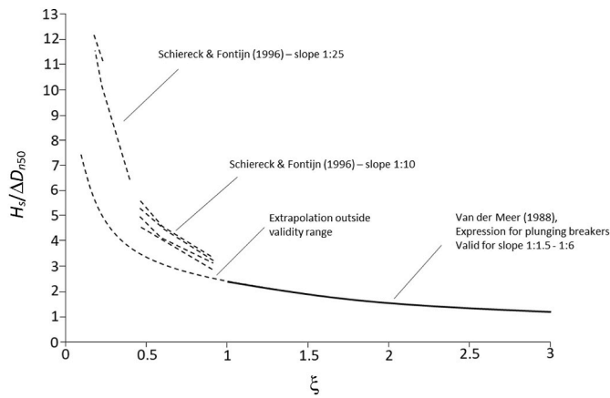
Fig. 1. Results of experiments carried out on a slope of 1:10 and 1:25 (Schiereck and Fontijn, 1996), where the vertical axis shows the stability number H_s/\Delta D_{n50} and the horizontal axis shows the surf-similarity parameter based on the mean wave period.
