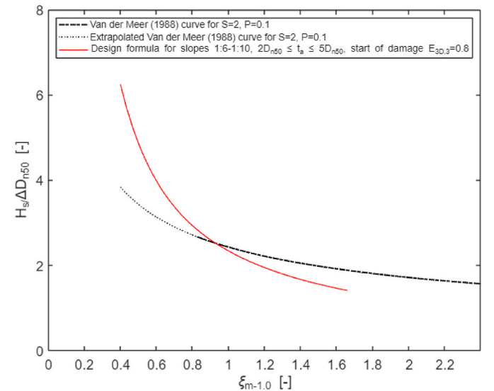
Fig. 17. Stability number for start of damage versus the surf-similarity parameter for mild rock-armour slopes (red curve) and for steep slopes according to Van der Meer (1988), both for structures in deep water.
