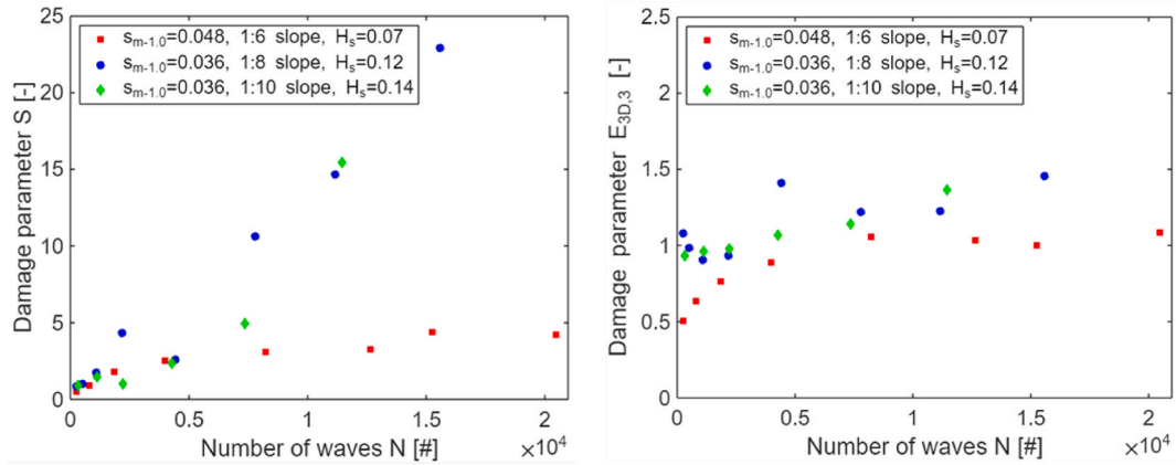
Fig. 11. Damage as function of the number of waves N for slopes 1:6, 1:8 and 1:10.
