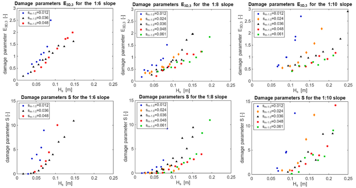
Fig. 10. (a) Damage S as function of the significant wave height H_s for varying wave steepness and slopes 1:6, 1:8 and 1:10 with a layer thickness t_d/D_{n50} = 2.5 (b) Damage parameter E_{3D,3} compared to significant wave height H_s for varying wave steepness and slopes 1:6, 1:8 and 1:10 with a layer thickness t_d/D_{n50} = 2.5 .
