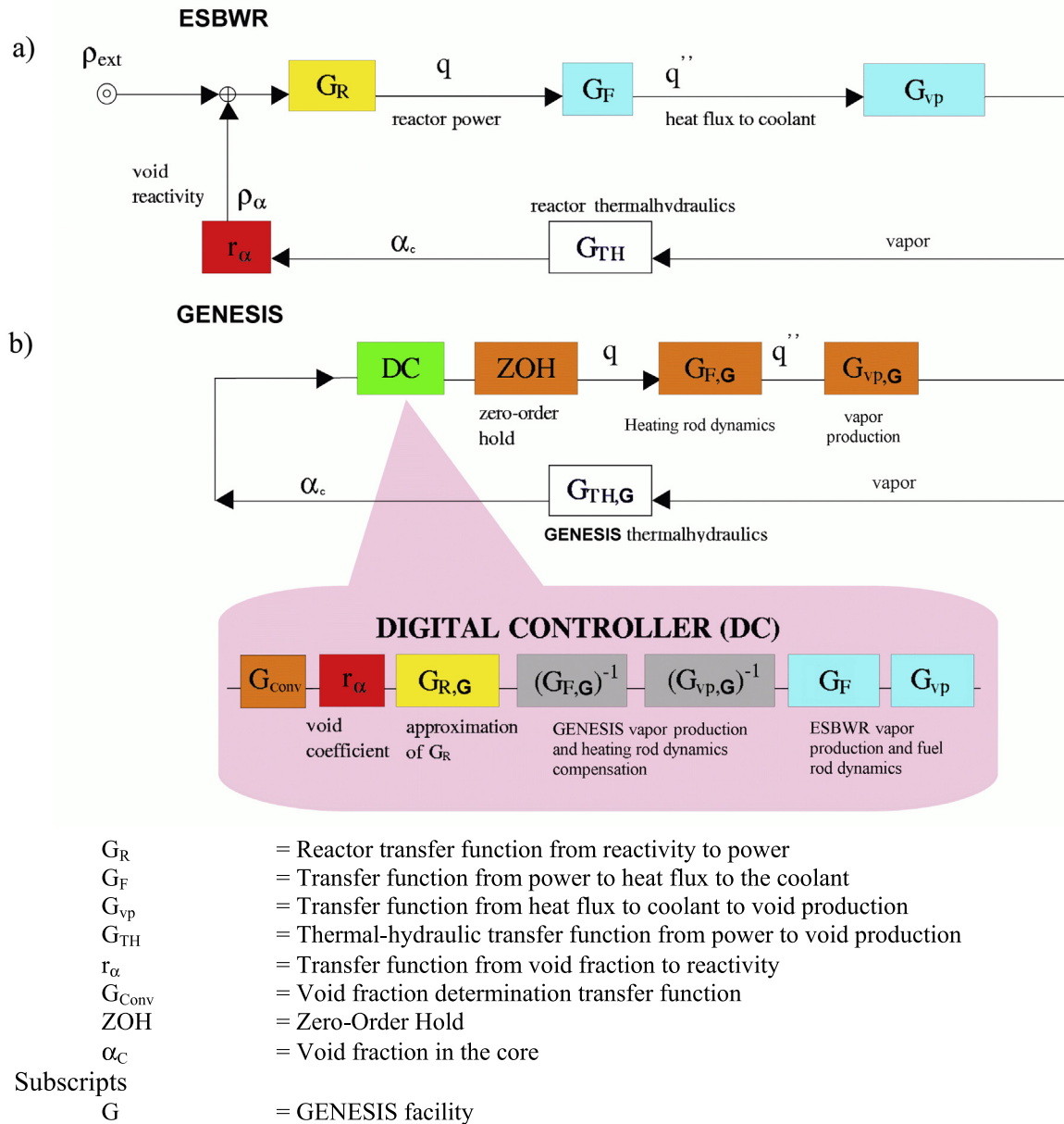
Fig. 2. (a) The feedback mechanism of the ESBWR and (b) the feedback system as implemented in the GENESIS facility (adapted from Zboray (2002)).
