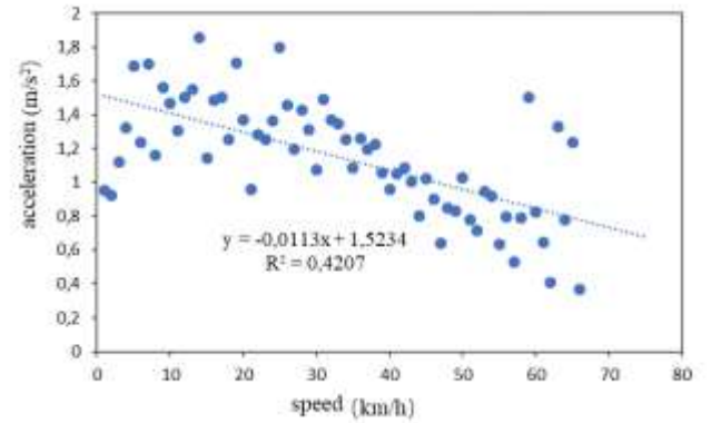
Fig. 7. Relation between speed and 95 percentiles of the acceleration for driver type 1
