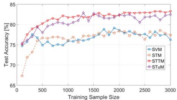
Fig. 7: Test accuracy of SVM, STM, STuM and STTM trained with different sample sizes.
