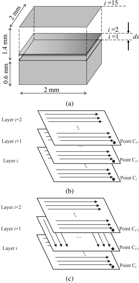
Figure 15: (a) Schematic illustration of (a) building 15 layers with a (b) fixed scanning strategy where the scanning directions are kept fixed for all the 15 layers and (c) alternating scanning strategy where the scanning pattern is rotated 90° in clockwise direction with respect to the scanning pattern of the previous layer.
