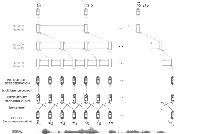
Fig. 3: The encoder architecture for speech-to-translation experiments was a three-layer bi-directional pyramidal LSTM, observing speech features computed by a one-layer convolutional network over the top of MFCCs.
