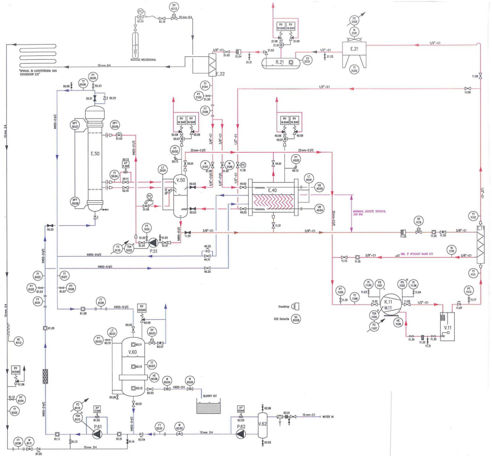
Figure 3: Process flow diagram of the system discussed in Chapter 4, containing a fluidized bed CO 2 -hydrate generator and a CO 2 -hydrate slurry cold storage vessel (V60). During the experiments reported in Chapter 4, the FBHE (E50) was used as generator. The system also includes a shell-and-plate generator (E40) which was not used during the experiments reported in this thesis
