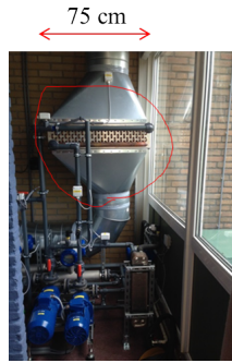
Figure 3.6: The installation of the tube-fin air cooler surrounded by a red circle. The two horizontal headers used to distribute the flow of hydrate slurry into 15 parallel circuits is clearly visible. Each vertical row of tubes is a different circuit.
