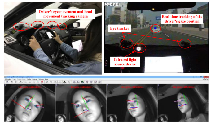
Fig. 5. Eye-tracking system.
