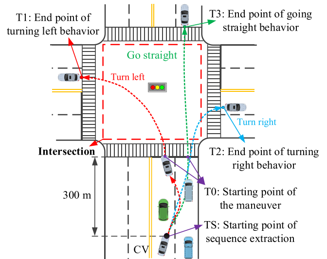
Fig. 8. Illustration of turning maneuvers at an intersection.
