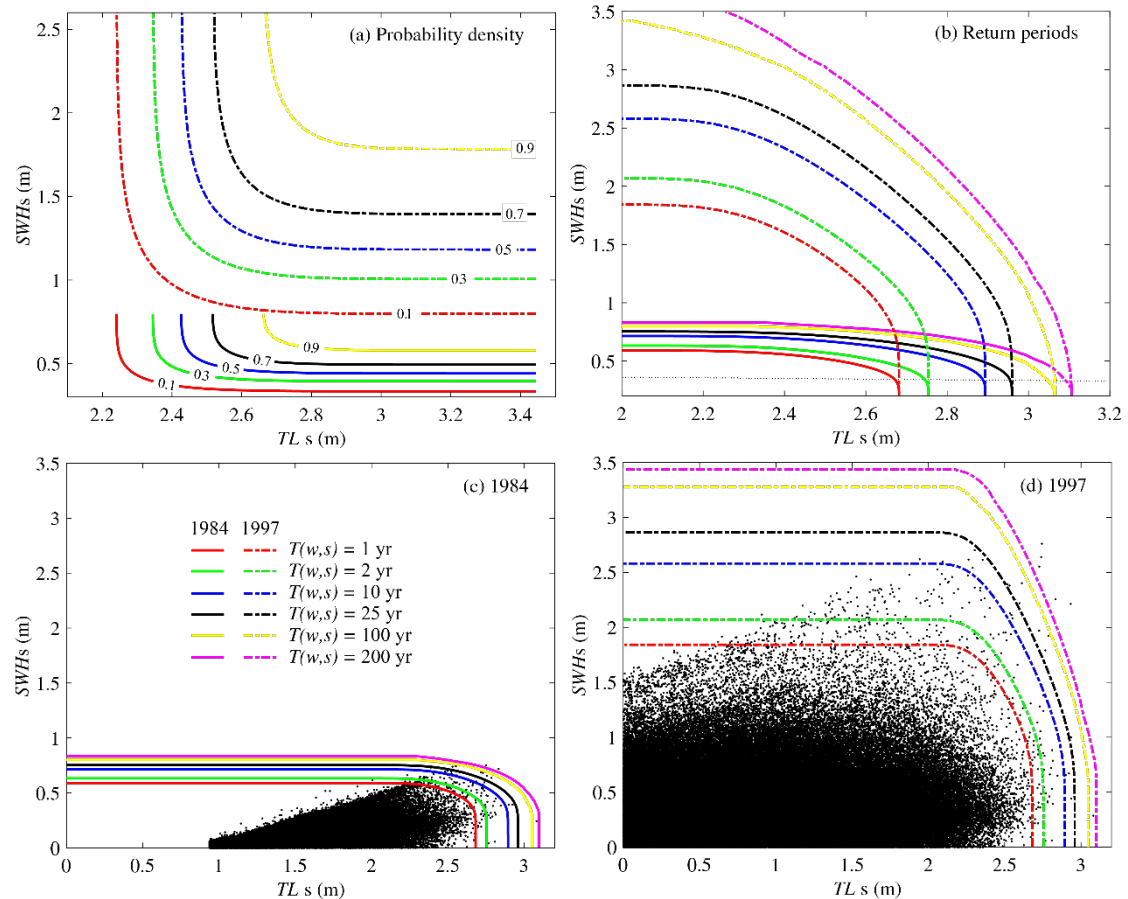
Fig. 7. Joint cumulative probability curves and joint return period curves for nearshore TL s and SWH s. (a, b) Comparison of joint cumulative probability F(w, s) curves and joint return period T(w, s) curves before and after reclamation; (c, d) the scatter plot of hourly TL s- SWH s for the past 40 years, and the comparison with the associated joint return period curves under the 1984 and 1997 intertidal profiles, respectively.
