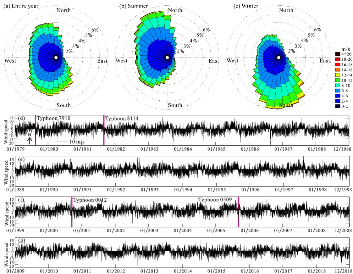
Fig. 4. Meteorological data of wind observed uninterruptedly during 1979 - 2018 recorded by the Fengxian Observation Station ( E121.45^{\circ} , N30.93^{\circ} ). (a, b, c) The wind rose of the entire year, the summer (May - October) and winter (November - April) periods. (d, e, f, g) The 6-hourly recorded wind magnitudes and directions from 1979 - 2018.
