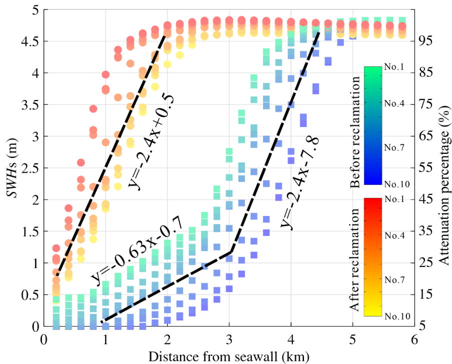
Fig. 11. Trend analysis of wave height reduction and attenuation ratio for the ten largest storms during the past 40 years. Colorbars denote the conditions before and after reclamation.
