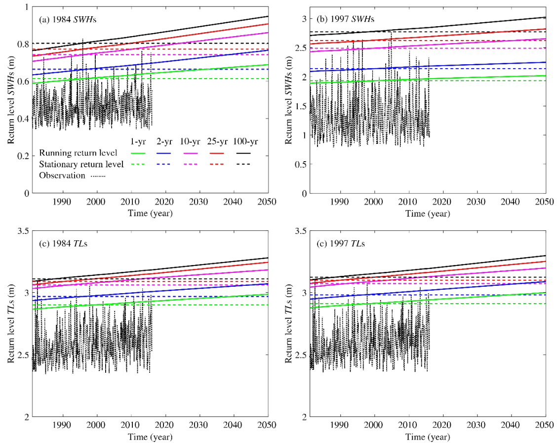
Fig. 13. Comparison of the running and stationary return levels before and after reclamation used for all years in coastal flood defense design.
