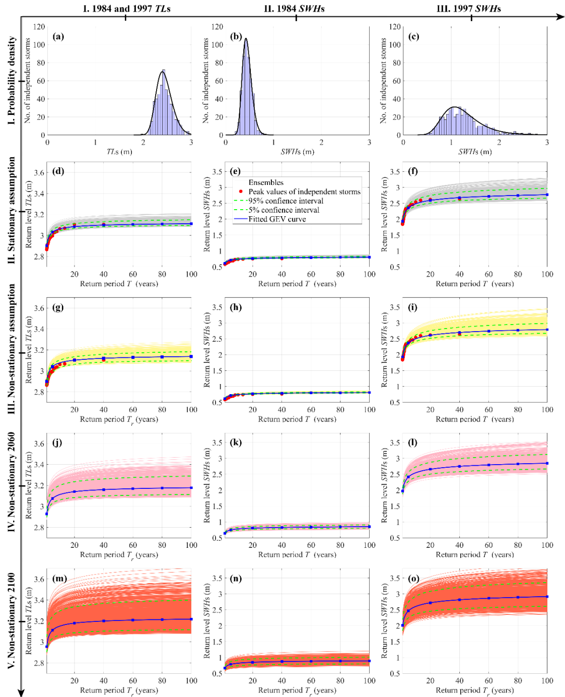
Fig. 6. Diagnostic plot of independent storms for the probability density (1 st row) and return levels vs. return periods with fitted GEV (generalized extreme value) curve (2 nd - 5 th row). Ensembles are used to provide the range of posterior probability bands and the confidence intervals (e.g., 5 % and 95 % quantiles). The 1 st column is the tidal levels (TLs) for both 1984 and 1997 tidal flat conditions, the 2 nd and 3 rd columns are the significant wave heights (SWHs) under 1984 and 1997 tidal flat condition, respectively. Stationary assumption: showing the return levels under the stationary distribution function; Non-stationary assumption: exhibiting the non-stationary return levels for the
