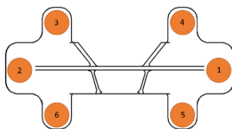
Fig. 7: Sequential spot welding sequence for the clip, skin and stringer joint.
