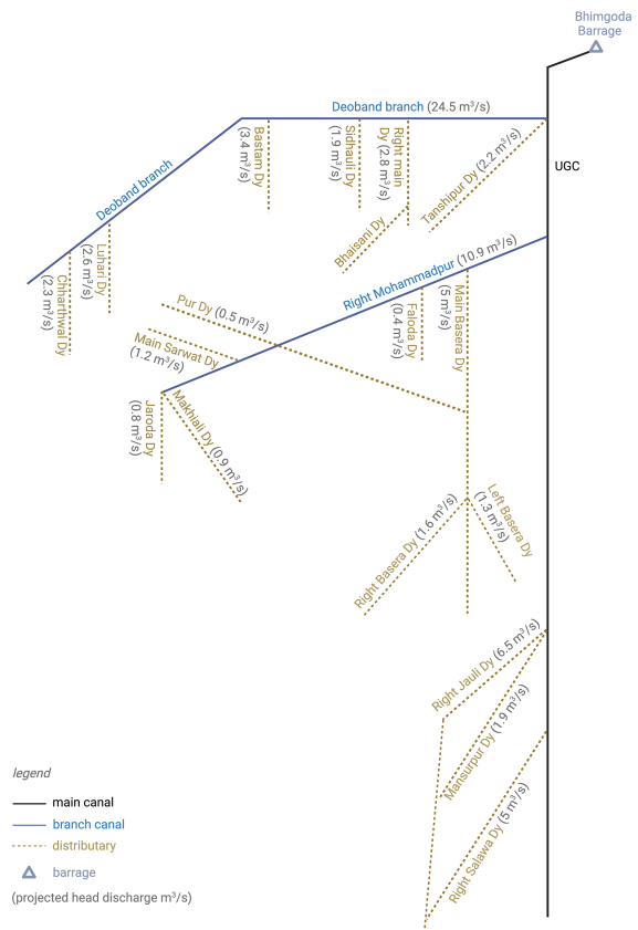
Figure A3. A schematic of the UGC main canal and its distributaries with their respective discharge capacities ( m^3 s^{-1} ).
