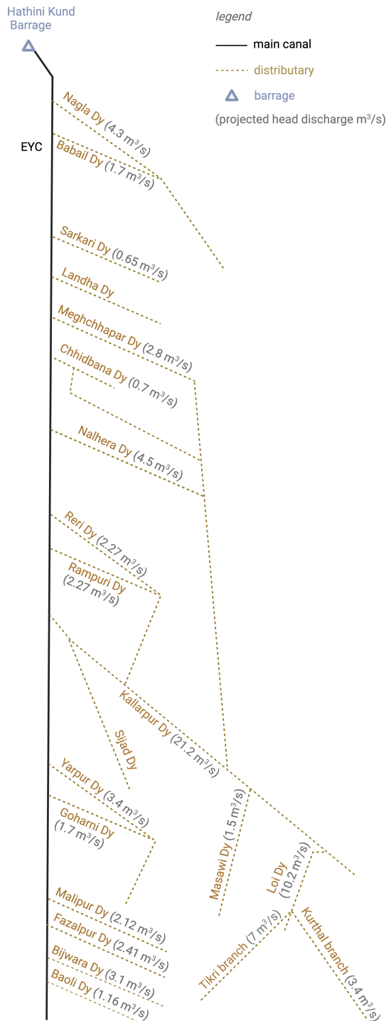
Figure A4. A schematic of the EYC main canal and its distributaries with their respective discharge capacities ( \text{m}^3 \text{s}^{-1} ).
