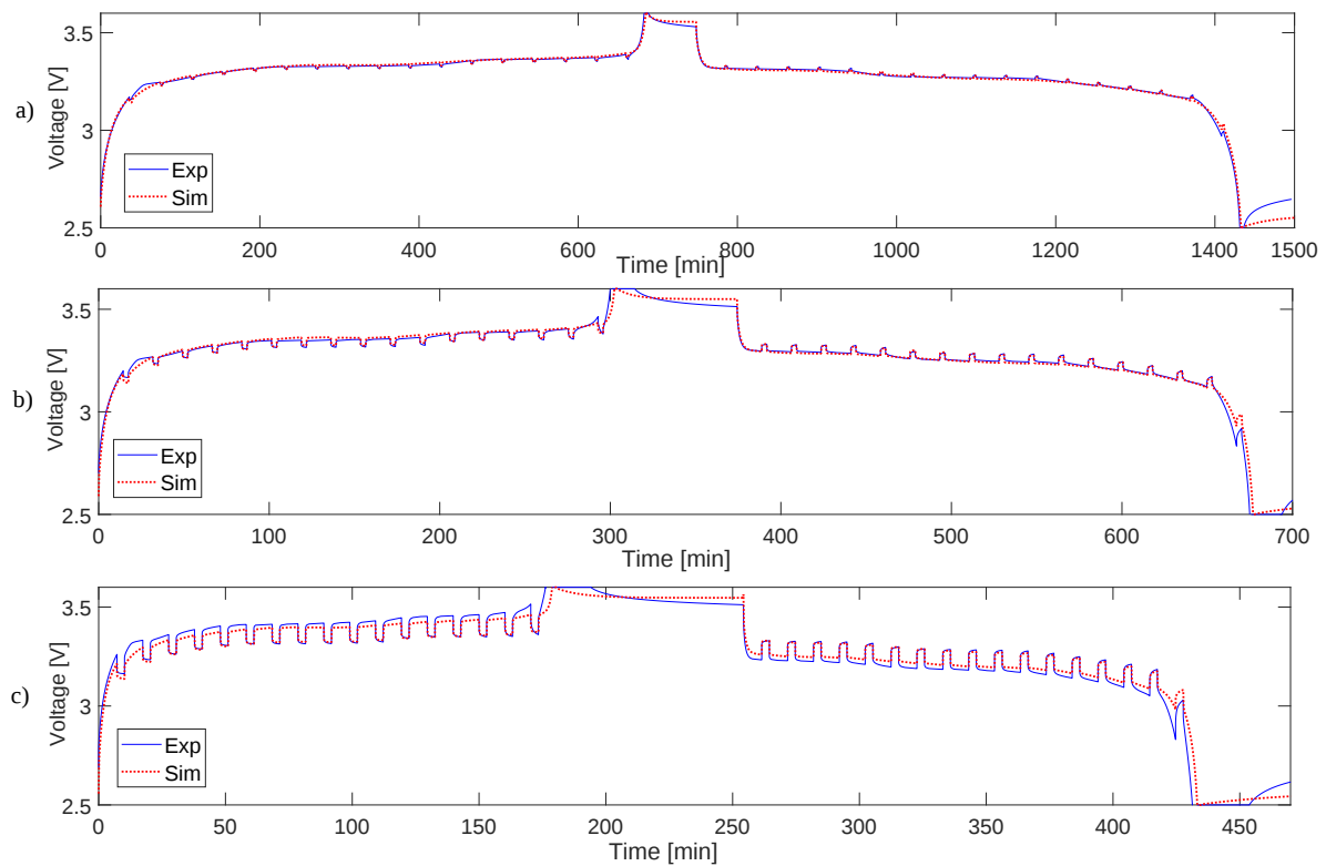
Figure 14. Comparison of experimental result and simulation result-LFP battery: (a) test with 0.1 C; (b) test with 0.25 C; and (c) test with 0.5 C.
