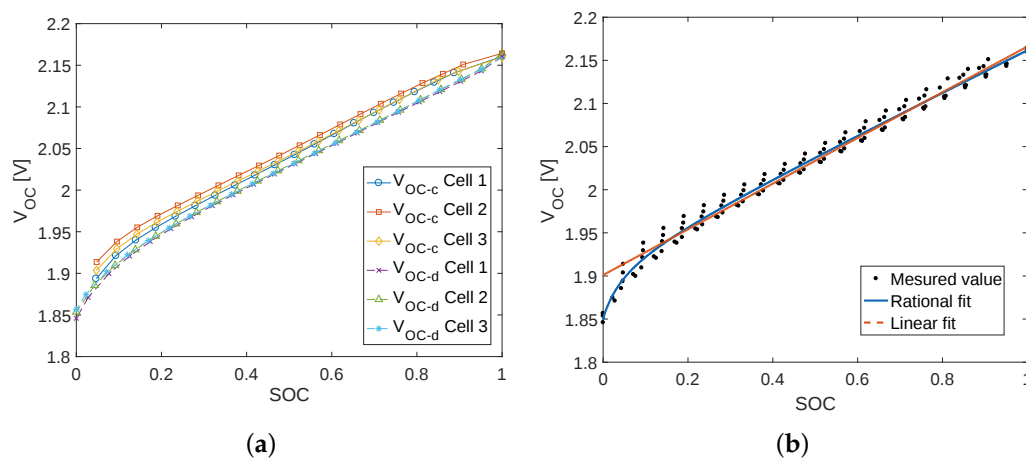
Figure 5. Measured open circuit voltage versus SOC of VRLA battery: (a) V_{OC} measured during charge and discharge separately; and (b) the measured data points and the fitted curves.
