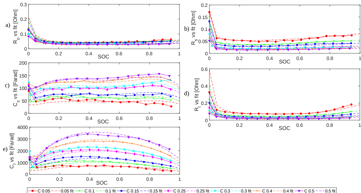
Figure 9. The values of RC elements and their fitted results: VRLA batteries during discharge.
