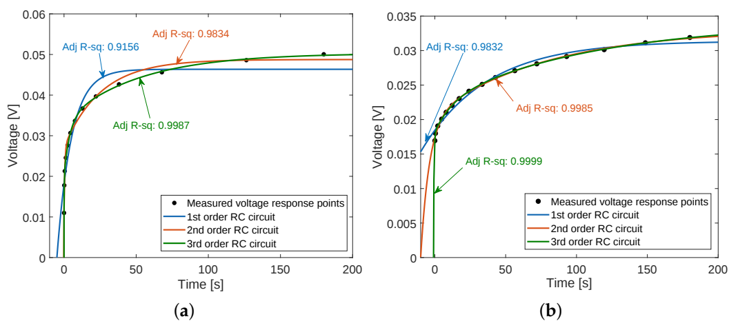
Figure 7. Comparison of accuracy with modelling battery into different orders of RC circuits: (a) VRLA battery; (b) LFP battery.
