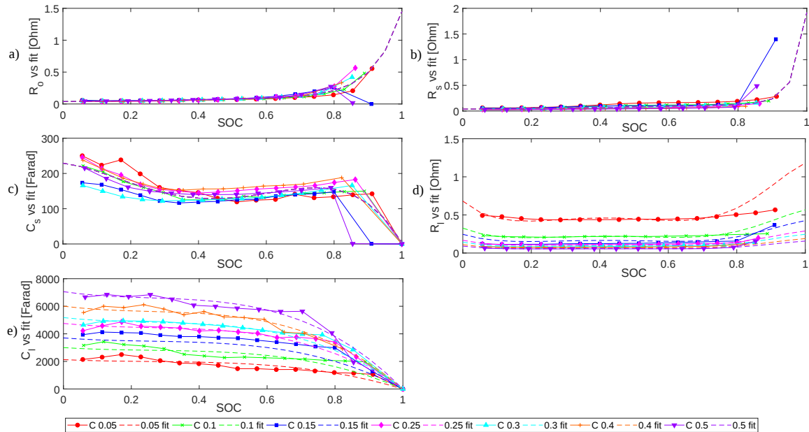
Figure 8. The values of RC elements and their fitted results: VRLA batteries during charge.
