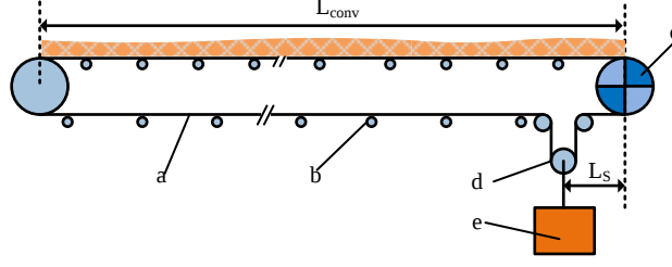
Figure 4: Typical belt conveyor geometry (Courtesy of [21])
