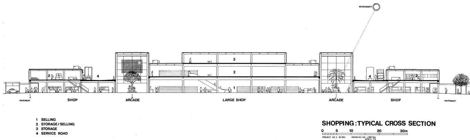
Figure 1. Schematic cross-section of Milton Keynes' shopping centre.
