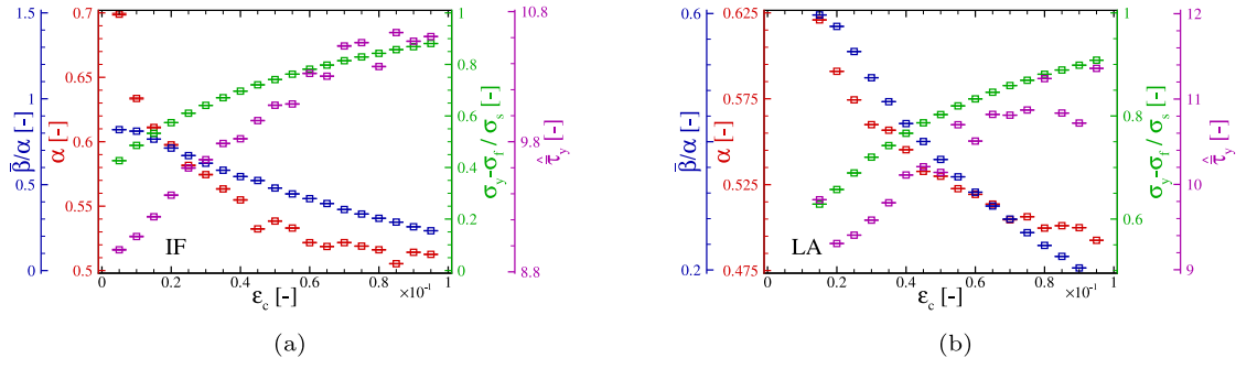
Fig. 8. The proportionality \alpha , scaled normalised work-hardening \beta/\alpha , normalised yield stress (\sigma_y - \sigma_t)/\sigma_s and scaled normalised yield stress \tau_y as functions of the cyclic principal true strain \epsilon_c for (a) IF and (b) LA. The error bars indicate the standard error in the experimentally obtained physical parameters.
