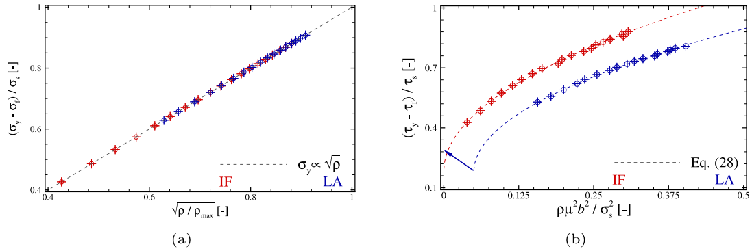
Fig. 10. (a) The scaled yield stress (\sigma_y - \sigma_t)/\sigma_s as a function of the square root of the scaled dislocation density \sqrt{\rho/\rho_{\max}} , and (b) the scaled shear flow stress (\tau_y - \tau_t)/\tau_s as a function of the normalised dislocation density \rho\mu^2b^2/\sigma_s^2 for IF and LA. The blue arrow indicates the original position of the origin of LA and the error bars indicate the standard error and the RMSE.
