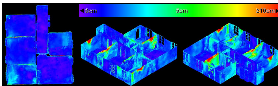
Fig. 8 Mean Hausdorff distance across all possible combinations for comparing two out of five triangle meshes of the complete apartment, where each triangle mesh has been captured with the Microsoft HoloLens (Hübner et al. 2019): nadir view (left) and two side views (center and right)
