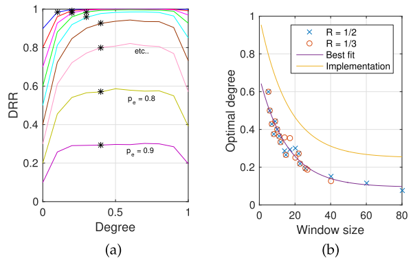
Fig. 7. Determining optimal degree value \Delta_{\text{optimal}} . (a) DRR for R=1/2 and W=10 for different frame loss probabilities when varying \Delta . The black crosses mark the lowest values for \Delta that give the maximal DRR for different frame loss probabilities. The largest of these values is \Delta_{\text{optimal}}=0.4 . (b) \Delta_{\text{optimal}} for different values for R and W . There is an exponential relation between \Delta_{\text{optimal}} and W . A relation with rounded-off fixed point coefficients is chosen as implementation.
