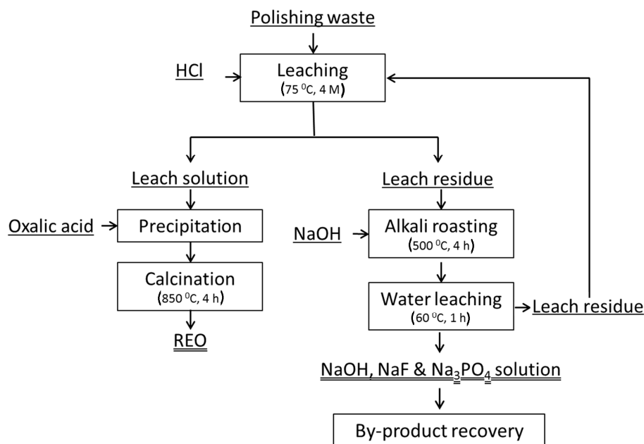
Figure 8. Flowsheet for complete recovery of REEs from polishing waste by acid-based process. This flowsheet shows that polishing waste was treated by acid leaching followed by alkali treatment.
