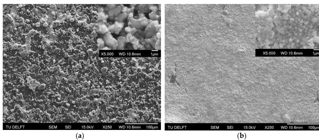
Figure 2. Scanning electron microscopy (SEM) images of the polishing waste samples: (a) sample A shows the coarser particles and (b) sample B shows the finer particles. Sample A is from plate glass polishing and sample B is from mirror polishing.
