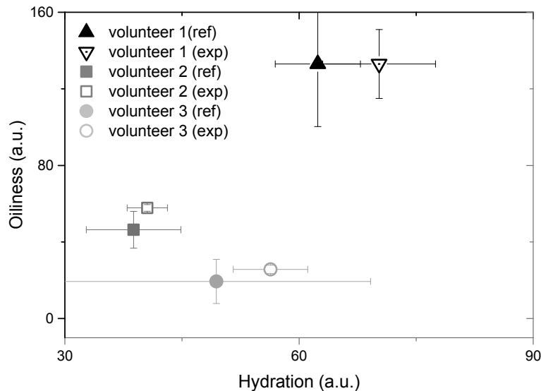
Figure. 2. Inter-individual variations of skin hydration and sebum levels measured on three persons on the forehead with Infrared spectroscopy and corresponding reference values obtained with Corneometer and Sebumeter.
