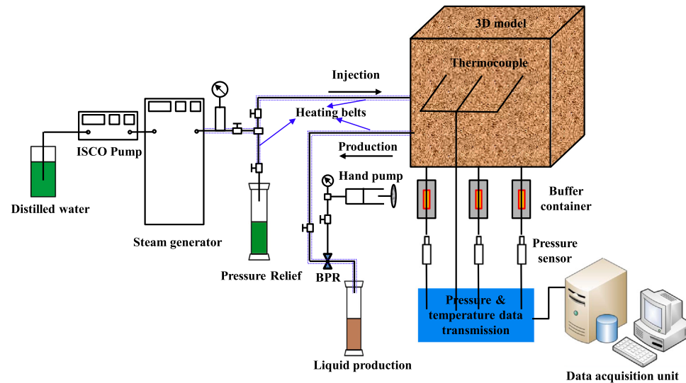
Fig. 1. 3D gravity drainage experiment apparatus.
