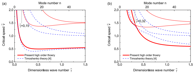
Figure 3. Resonant speeds for h/R = 0.1, \bar{k}_c = 0.1 : (a) \bar{k}_r = 0.01 ; (b) \bar{k}_r = 0.5 .
