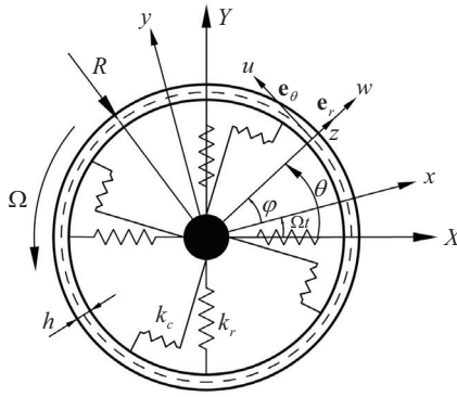
Figure 1. A rotating ring on an elastic foundation
