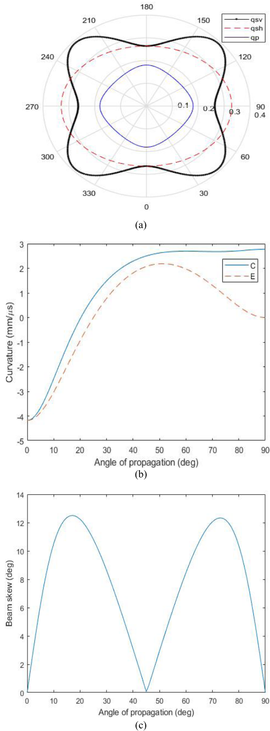
Fig. 4. Beam field using (a) slowness surfaces, (b) slowness surface curvatures C and E , and (c) beam skew.
