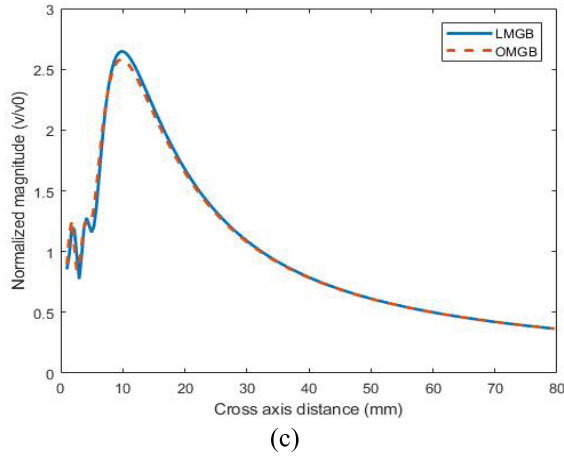
Fig. 6. Beam field at a steering angle of 0^\circ using (a) OMGB, (b) LMGB, and (c) on-axis magnitude.
