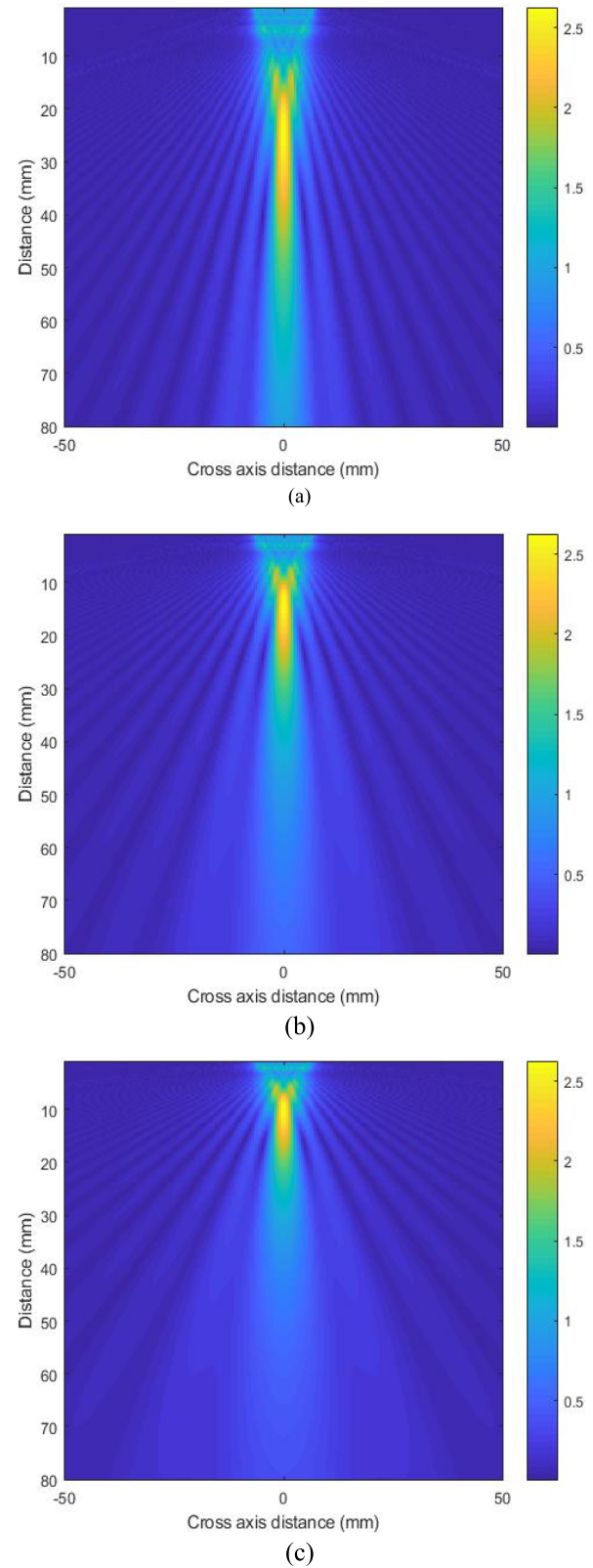
Fig. 5. Beam field: (a) C = E = 0 , (b) C = E = -2.5 \text{ mm}/\mu\text{s} , and (c) C = E = -4.9 \text{ mm}/\mu\text{s} .
