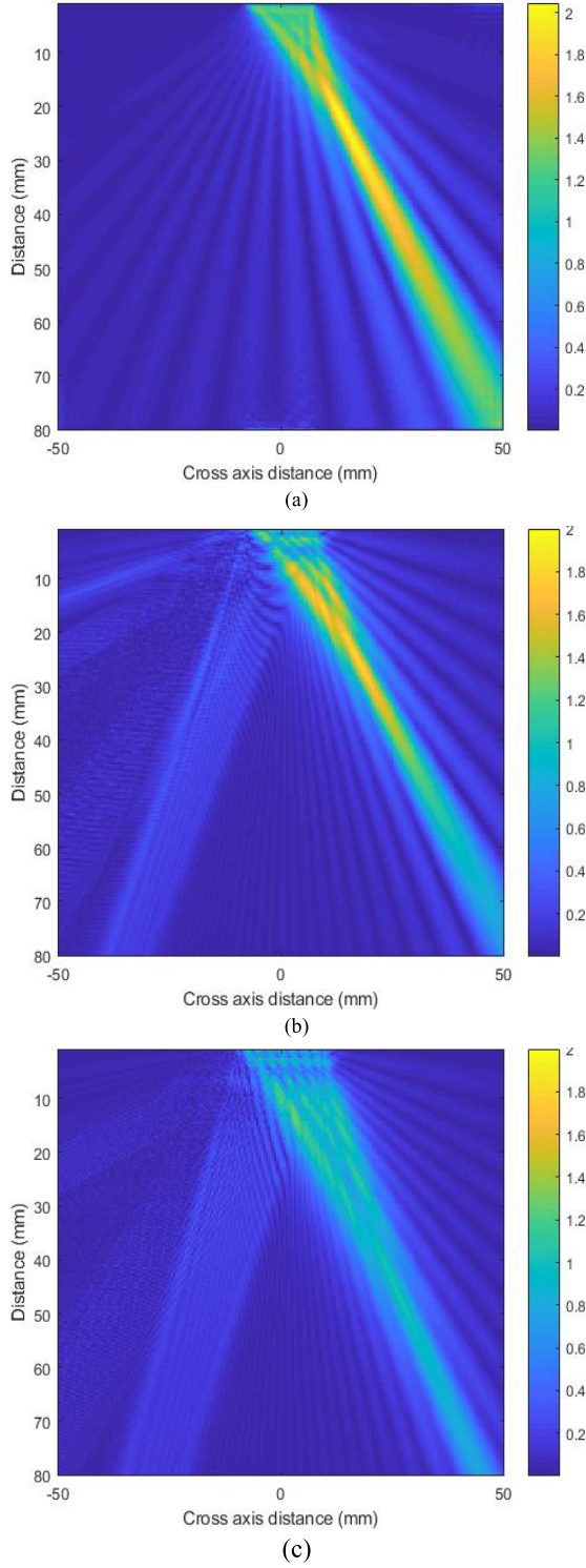
Fig. 8. Beam field using (a) COMSOL, (b) LMGB, and (c) OMGB for a steering angle of 30°.
