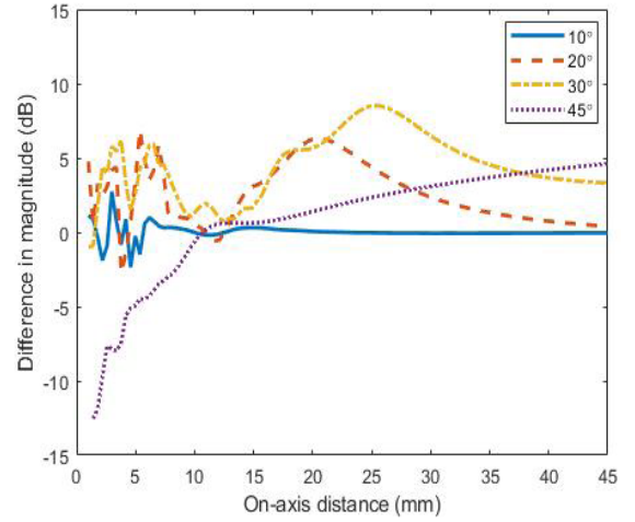
Fig. 11. Difference in on-axis amplitudes (dB) for different steering angles between the LMGB and OMGB models.
