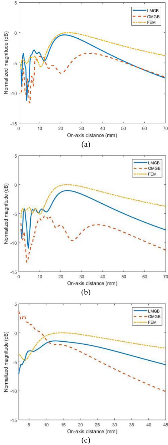
Fig. 10. On-axis beam fields calculated using the analytical and numerical models for the steering angles of (a) 20°, (b) 30°, and (c) 45° in the decibel (dB) scale.
