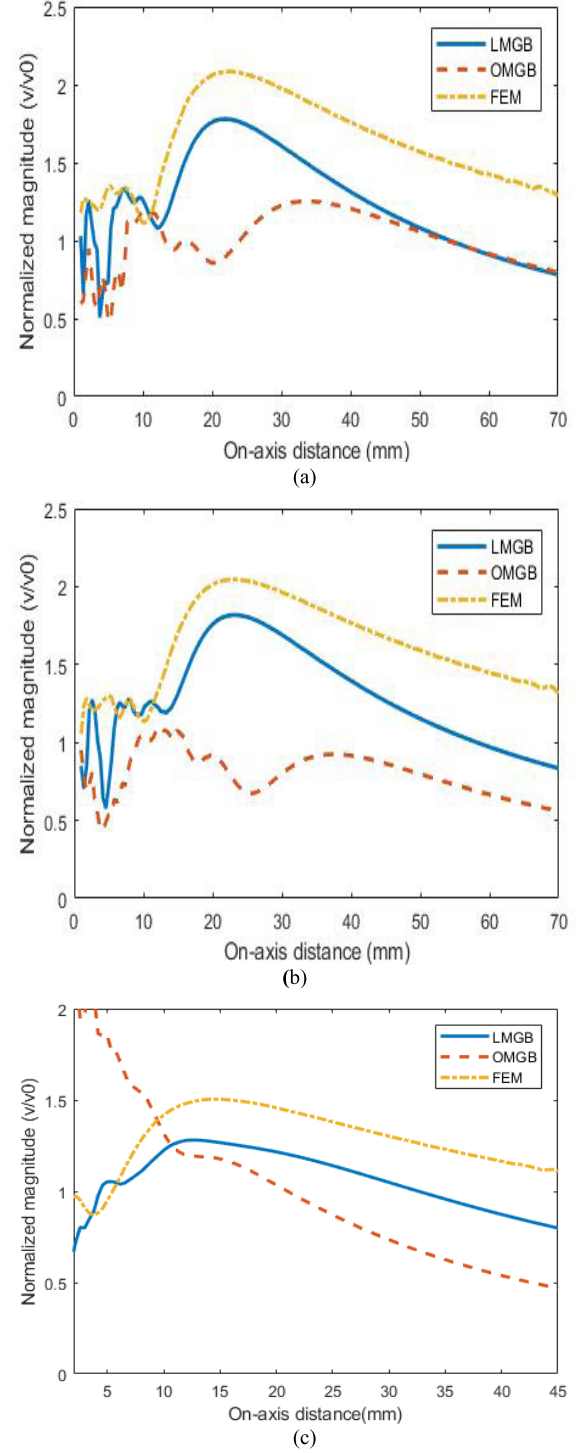
Fig. 9. On-axis beam fields calculated using the analytical and numerical models for the steering angles of (a) 20°, (b) 30°, and (c) 45°.
