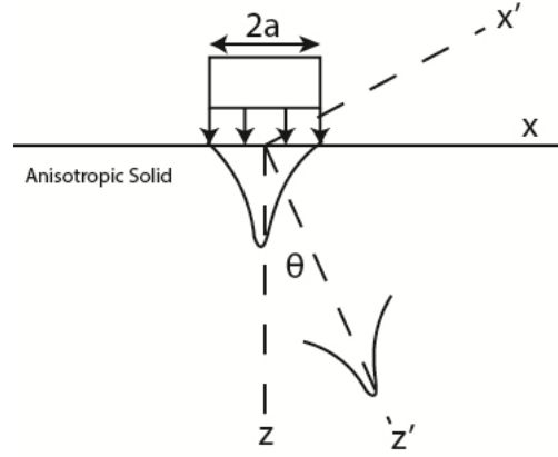
Fig. 1. Transducer radiating a Gaussian beam at an angle \theta (group velocity direction).
