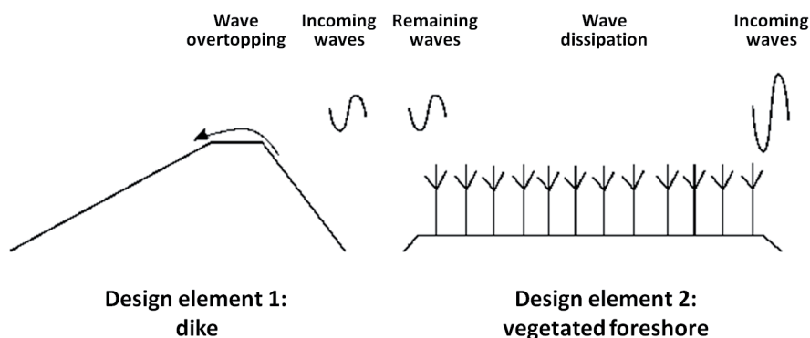
Figure 4. Visualisation of design elements for the foreshore-dike (hybrid) flood defence Noordwaard.
