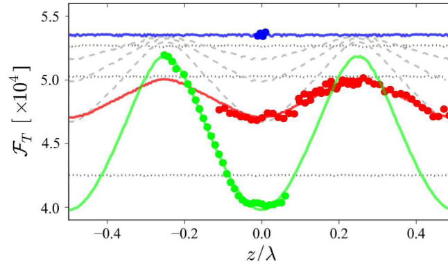
FIG. 6. Plot of the cavity finesse, \mathcal{F}_T versus membrane position along the cavity axis. Red-symbols represent data for a circular-membrane, 1.2 mm diameter, and 97 nm thickness. Red-line represents the best fit with fitting parameters \bar{n}_I = (1.97 \pm 0.08) \times 10^{-6} and \bar{\sigma}_{\text{opt}} = (287 \pm 4) pm, and with the following fixed parameters: the membrane thickness L_d = 97 nm, the real part of the refractive index n_R = 2.021 , the cavity length L = 9.03 cm, the wavelength \lambda = 1064 nm, and the empty-cavity finesse \mathcal{F}_v = 53500 \pm 100 , which is evaluated as mean value of the data shown as blue-symbols. Green-symbols represent data for a square-membrane, 1 mm side, 50 nm thickness by Norcada. The green-line is the fitting with parameters n_I = (1.0 \pm 0.01) \times 10^{-5} and \sigma_{\text{opt}} = (280 \pm 10) pm. Dashed-gray (dotted-gray) curves represent theoretical expectation for the circular membrane with parameters fixed as \sigma_{\text{opt}} = 0 ( n_I = 0 ) and n_I/\bar{n}_I = .5, 1, 2 ( \sigma_{\text{opt}}/\bar{\sigma}_{\text{opt}} = .5, 1, 2 ), from upper to lower curve. They demonstrate the different contribution of absorption and roughness to the finesse behaviour upon membrane position.
