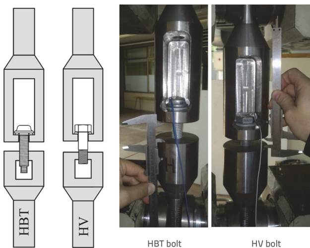
Figure 12. Test layout for bolt calibration
