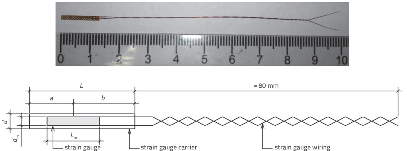
Figure 8. BTM-6C strain gauge
