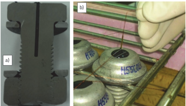
Figure 9. a) Positioning strain gauge in HV bolt; b) embedding rectangular bended strain gauge into HBT bolts
