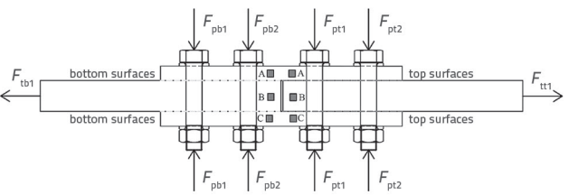
Figure 5. Labelling of forces acting on specimens and tensometer measurement positions
