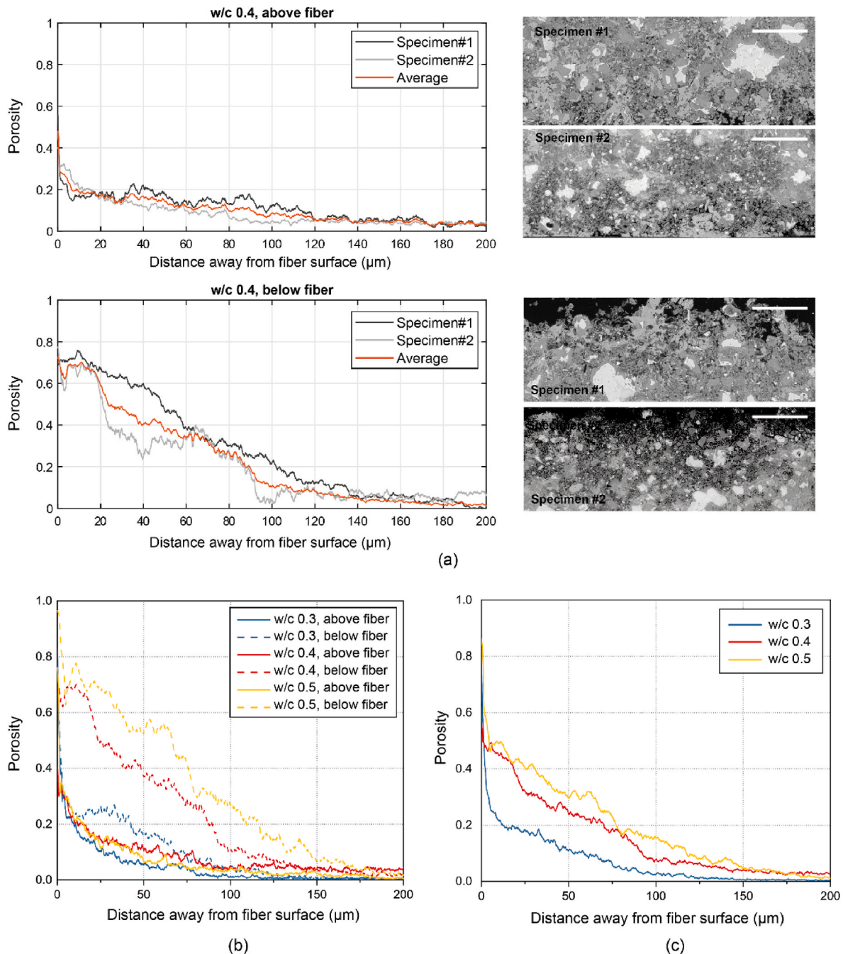
Fig. 8. Volume fraction of pores at different distances from the fiber/matrix interface for: (a) 2 specimens with same w/c ratio, (b) averaged upper and lower ITZs for all tested w/c ratios and (c) normalized ITZ for all tested w/c ratios.
