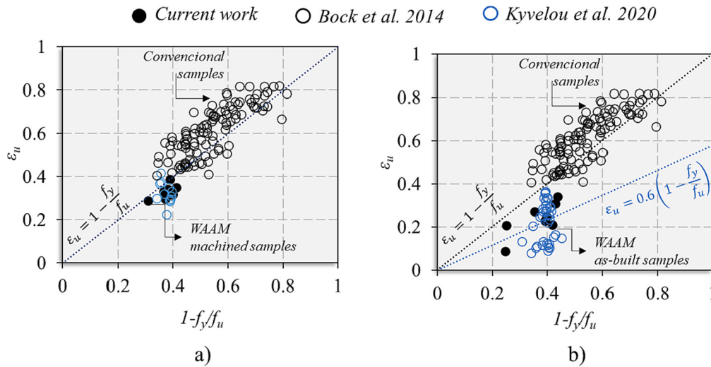
Fig. 15. – Comparison between the evolution of the \varepsilon_u values with the 1-f_y/f_u ratio for different austenitic stainless steels produced by conventional manufacturing techniques (white circles) and by WAAM process (black and blue circles) in the (a) machined and (b) as-built condition. (For interpretation of the references to colour in this figure legend, the reader is referred to the web version of this article.)
