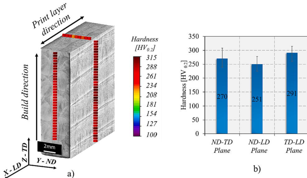
Fig. 9. (a) Hardness distribution map and (b) hardness average values along the TD-LD, ND-LD and ND-TD planes.
