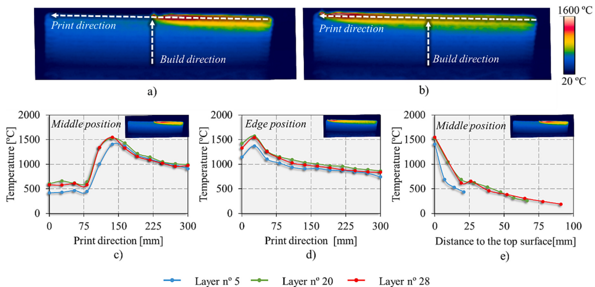
Fig. 6. Schematic representation of the temperature measurement sites along the building and printing directions, during the printing of layers 5th, for when the torch was in the (a) middle and (b) edge position of the wall. Temperature distribution along the printing direction for when the torch was in the (c) middle and (d) edge positions. Temperature distribution along the building direction (e) for when the torch was in the middle position.
