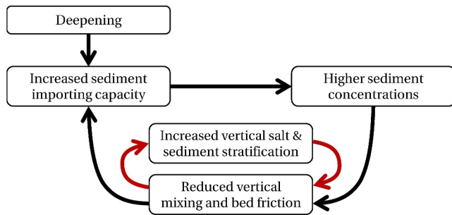
Figure 8. Feedback process enabling the regime shift. Adapted with some changes from Dijkstra, Schuttelaars, Schramkowski, and Brouwer (2019) and Lin et al. (2021).
