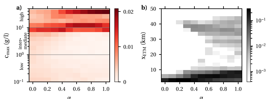
Figure 11. Two-dimensional histogram of the sensitivity study for Q , c_{\text{sea}} , and w_{s,0} plotted against the bed level parameter \alpha . Colors indicate the fraction of experiments in its respective two-dimensional bin. Panel a plots the histogram for the subtidal near bed concentration in the ETM. Panel b plots the histogram for the ETM location.
