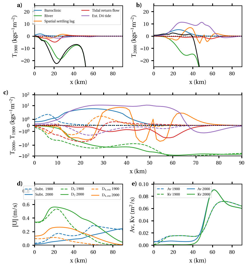
Figure 9. Panels (a–c) show the 5 most dominant contributions to the transport capacity and the sum of all contributions (black line). Panels a, b show the results for the default case for neap in 1900 and 2000. Panel c shows the same results for 1900 (dashed) and 2000 (solid) in one plot and on a logarithmic scale. Panel d shows the depth-averaged subtidal velocity and tidal D_2 and D_4 velocity amplitudes ( |u| ) for the default neap case in 1900 and 2000. Panel e shows the eddy viscosity ( A_v ) and eddy diffusivity ( K_v ) for the default neap case in 1900 and 2000.
