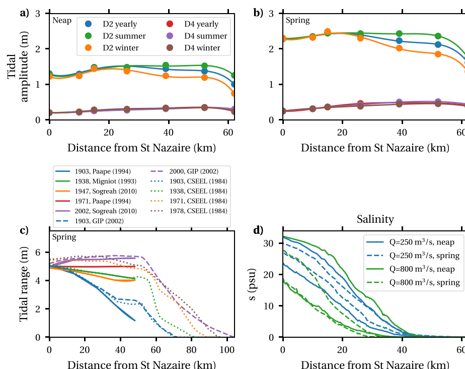
Figure 3. (a–b) Observed tidal amplitudes filtered from tidal gauge measurements using complex demodulation (Jalón-Rojas et al., 2016). (c) tidal range during low discharge and spring tide over the 20th century (GIP, 2002; Migniot, 1993; Paape, 1994; Sogreah, 2010). (d) 2008–2018 3D modeled average salinity in the thalweg for two discharge classes and spring and neap conditions. For each conditions, two lines are plotted representing surface and bottom salinity.
