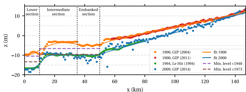
Figure 2. Thalweg level of the Loire upstream from Saint-Nazaire. Data is presented from between 1900 and 2009 (GIP, 2004, 2011, 2014; Le Hir, 1994). Additionally, the solid lines show the smooth fits used in the model for the 1900 and 2000 cases. Dashed lines show data of threshold bed levels specified by dredging operations (see Table 1, Sogreah (2006)).
