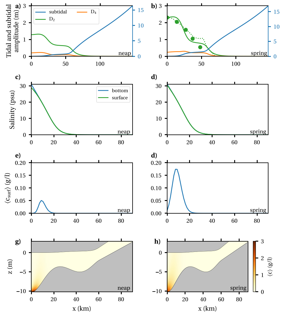
Figure 6. As Figure 5 for the year 1900 case. The spring D_2 tidal amplitude panel (b) is compared to 0.5 \times the observed tidal range as reported by Paape (1994) (circles) and CSEEL (1984) (dotted).
