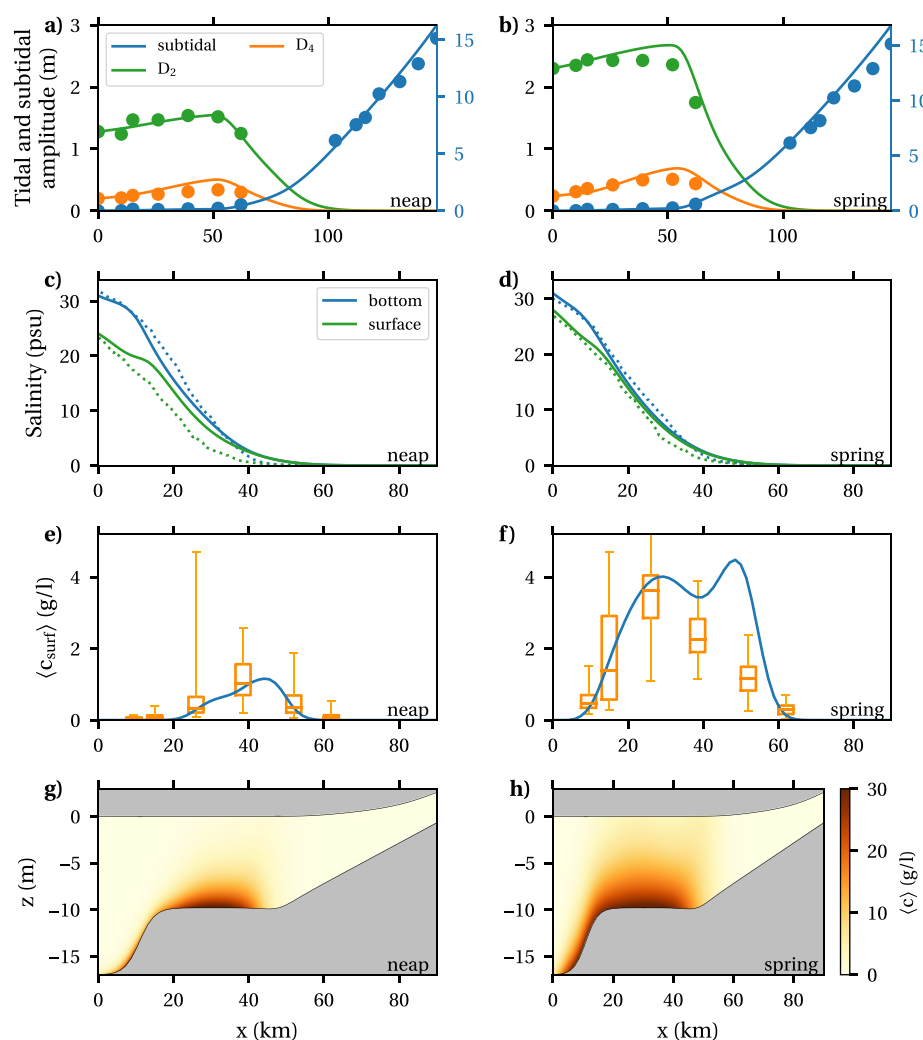
Figure 5. Model results for the default 2000 case for neap (left) and spring (right). Panels (a, b) show the surface amplitude compared against observations for the summer season (circles). The left vertical axis is for the D_2 and D_4 signals, while the right axis is for the subtidal set-up. Panels (c, d) show the salinity at the surface and bottom comparing our model results (solid lines) and thalweg concentrations from a 3D complex model (dotted lines). Panels (e, f) show the subtidal surface sediment concentration plotted against a boxplot with SYVEL observations near the surface for low discharges (Jalón-Rojas et al., 2016). Finally, panels (g, h) show along-channel sections of the modeled subtidal concentration.
