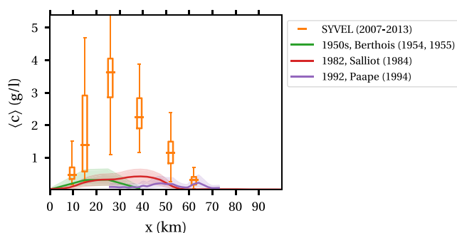
Figure 4. Evolution of the tidally averaged sediment concentration \langle c \rangle near the water surface for low river discharges and spring tidal conditions since the 1950s. The green curve is an estimate of tidally averaged concentrations in the 1950s from instantaneous measurements (Berthois, 1954, 1955). The shaded area is used to indicate the observed spread. The most recent turbidity measurements are from the SYVEL network (Jalón-Rojas et al., 2016).
