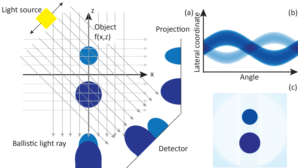
Figure 1.2: Schematic Illustration of the basic principle of computed tomography. (a) Parallel beam geometry for three different angles and the resulting projections at the detector. The unknown object is f(x,z) . (b) Visualization of the projections in a sinogram. (c) Reconstruction of the object from the projections using filtered back projection.
