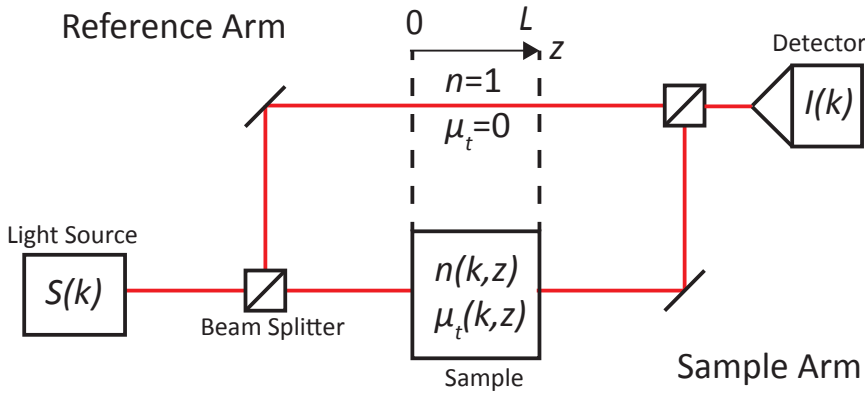
Figure 2.1: Schematic diagram of the Fourier-domain transmission OCT system. I(k) : detected intensity at the spectrometer, L : length of the sample, n(k,z) : refractive index of the sample, \mu_t(k,z) : total attenuation, S(k) : source intensity
