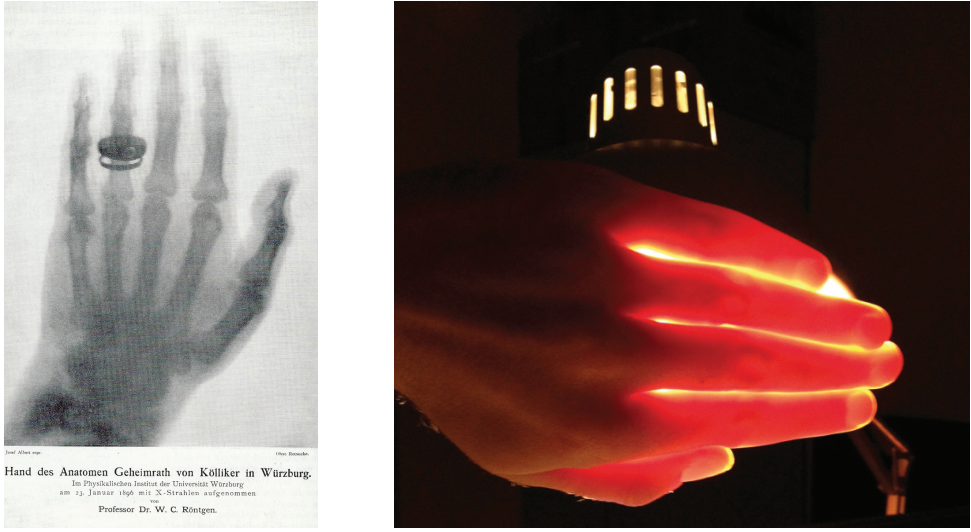
Figure 1.8: Left: X-ray image of the hand of Albert von K  lliker made by Wilhelm R  ntgen [26]. Right: optical transmission image of the human hand. [27] as a function of wavelength.
