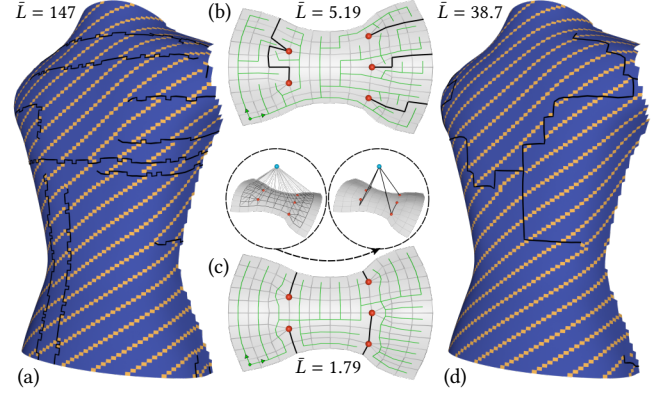
Fig. 11. Tiling the designed SJJ patterns onto a stitch mesh. Tiling by direct flooding ((a) & (b)), where the order of flooding has been illustrated as green paths shown on the patch in (b). The bold black curves illustrate the boundaries of neighboring stitches with incompatible SJJ patterns – discontinuity. To reduce the length of incompatible curves, we compute them by constructing a minimal spanning tree (MST) to connect all apexes (shown as red points in (b) & (c)) and use all boundary nodes as a common virtual node (see the blue point shown inside the circles of (c)). As a result, the discontinuity can be significantly reduced (see the tiling result shown in (d)). The SJJ pattern shown in Fig. 4 is employed in (a) and (d) to demonstrate the discontinuity. The total length of incompatible boundary curves \bar{L} is also given for every model.
