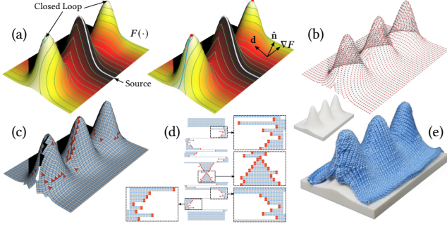
Fig. 7. Steps for generating knittable stitch meshes on a given surface: (a) Isocontours of a geodesic distance-field F(\cdot) are used as wale curves with segments having nearly equal length. The input mesh will be cut if there are closed wale curves. The resultant wale curves are sorted according to their values of F(\cdot) . (b) Optimal quadrangles / triangles are constructed between neighboring wale curves. (c) Courses are traced out and sorted on a stitch mesh to generate the final knitting map. (d) The physical knitting result can be generated by following the knitting map, where the stitch size is 3.5\text{mm} \times 2.8\text{mm} in this example. (e) The physical knitting result.
