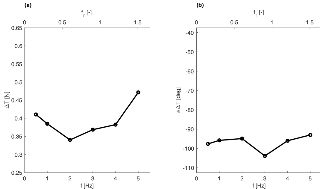
Figure 12. Thrust variation as a function of the yaw motion frequency for the rated wind speed of U = 4 \text{ m s}^{-1} and the same value of motion velocity of 19^\circ \text{ s}^{-1} : (a) experimental amplitude and (b) phase.
