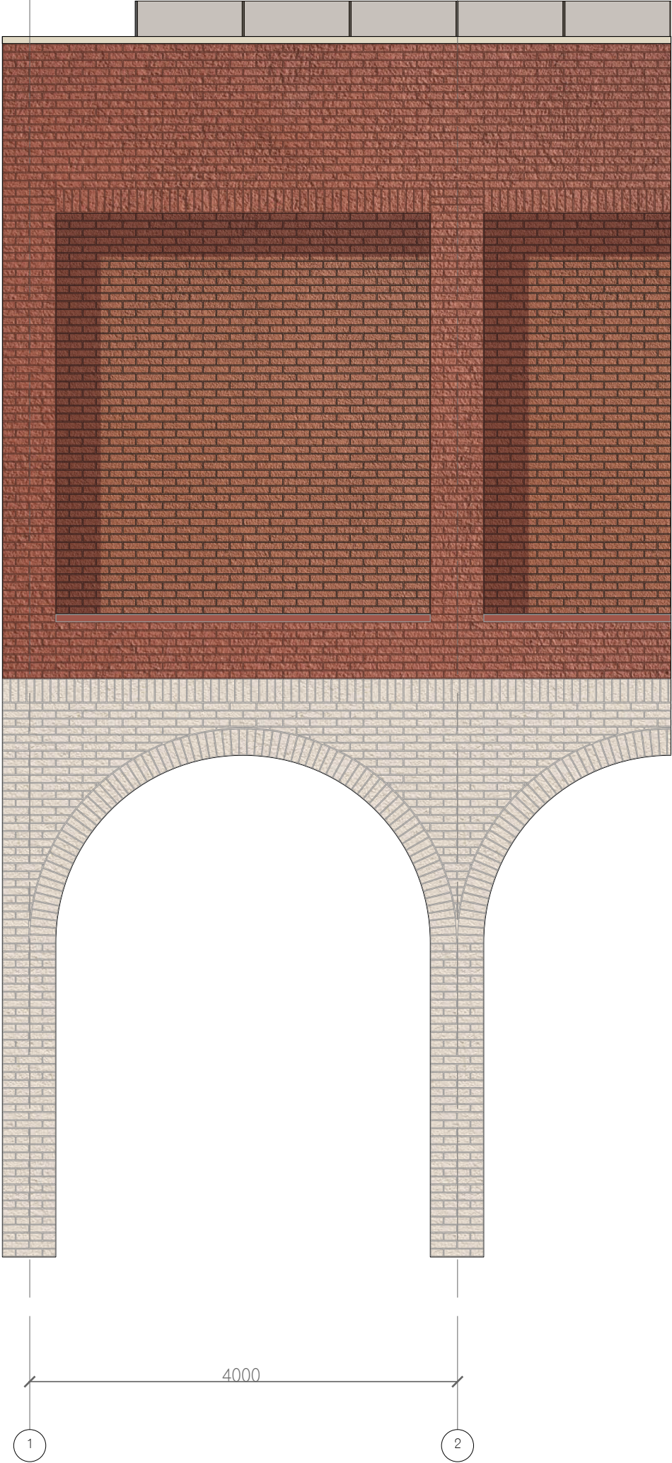
FACADE DETAIL SCALE 1:50
