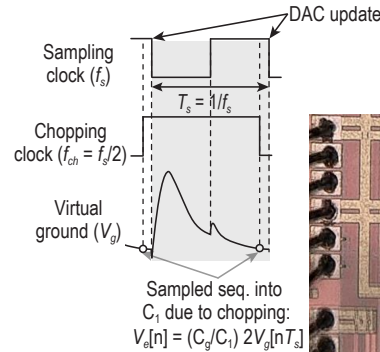
Fig. 3: Sampled sequence due to chopping.
