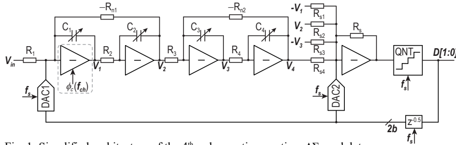
Fig. 1: Simplified architecture of the 4 th order continuous-time \Delta\Sigma modulator (input feed-ins are not shown).
