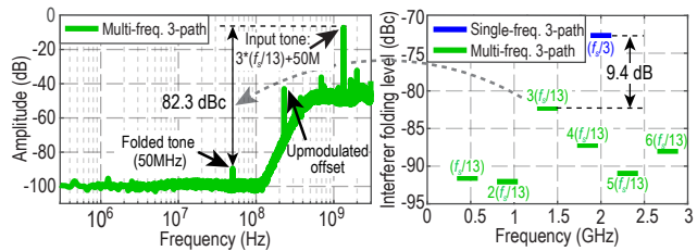
Fig. 7: Measured spectrum with out-of-band interferer (RBW=10kHz).
