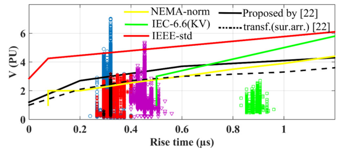
Fig. 17. Comparison of restrikes with different standard (color: blue circle = without SPD, red star = with arrester, green square = with snubber and purple triangle = with choke)
