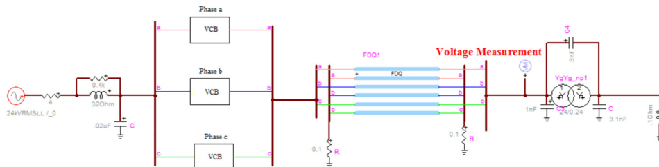
Fig. 2. EMTP-RV wind turbine power network model used for simulation.
