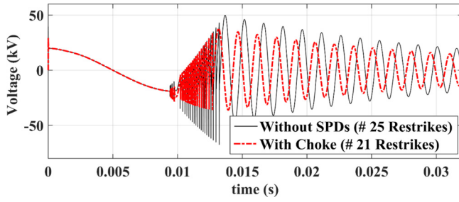
Fig. 9. Transformer voltage with and without a choke.
