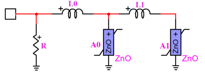
Fig. 3. Simplified surge arrester model.
