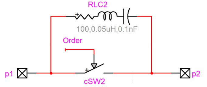
Fig. 1. VCB opening model in EMT-P-RV.
