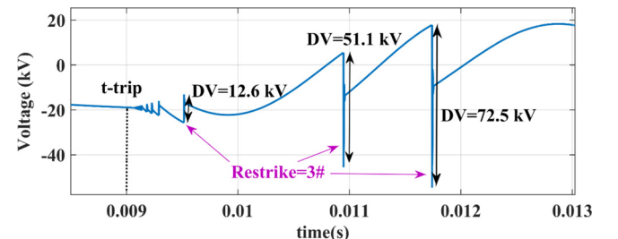
Fig. 13. Waveform of the high voltage side of the transformer.
