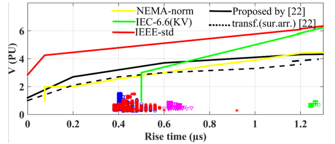
Fig. 23. Comparison of prestrikes with different standard (color: blue circle = without SPD, red star = with arrester, green square = with snubber and purple triangle = with choke).
