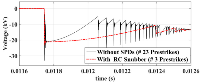
Fig. 7. Transformer voltage with and without RC snubber for VCB closing (magnified in time).
