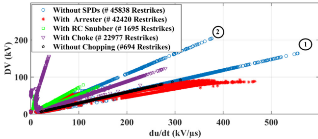
Fig. 16. Scatter plot diagrams of recorded restrikes.
