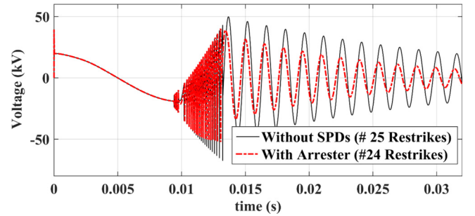
Fig. 4. Transformer voltage with and without surge arrester.
