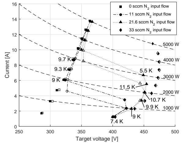
Fig. 2. LLS801 I - V relationships in the low flow regime. The argon input flow is 55.4 sccm and the argon partial pressure 0.6 Pa. Deposited thin films have an added T_c value. Isopower curves are depicted by the dashed lines. Upward power sweeps are indicated by the filled symbols, downward power sweeps by the unfilled symbols.
