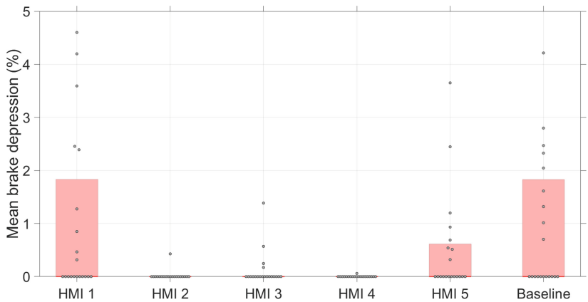
Fig. 3. Braking effort per HMI condition (Experiment 1).
