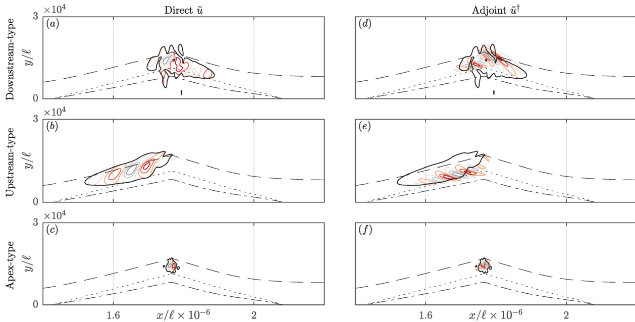
FIG. 4. Initial conditions corresponding to the most unstable eigensolution for upstream-type ( c_f/u_e = 0.557 ) and downstream-type ( c_f/u_e = 0.587 ) modes at \beta_{ud} and for apex-type mode ( c_f/u_e = 0.615 ) at \beta_a . Colored lines from minimum (gray) to maximum (red) with \Delta = 2/9 for isocontours of (a)–(c) \mathcal{R}(\tilde{u})/|\tilde{u}|_{\max} (direct solution) and (d)–(f) \mathcal{R}(\tilde{u}^\dagger)/|\tilde{u}^\dagger|_{\max} (adjoint solution). (a)–(f) Isocontour of |\tilde{u}|/|\tilde{u}|_{\max} (solid black, level: 1/9), \bar{U} = 0.9u_e -isocontour (dashed black), dividing streamline (dotted black), and \bar{U} = 0 -isocontour (dash-dotted).
