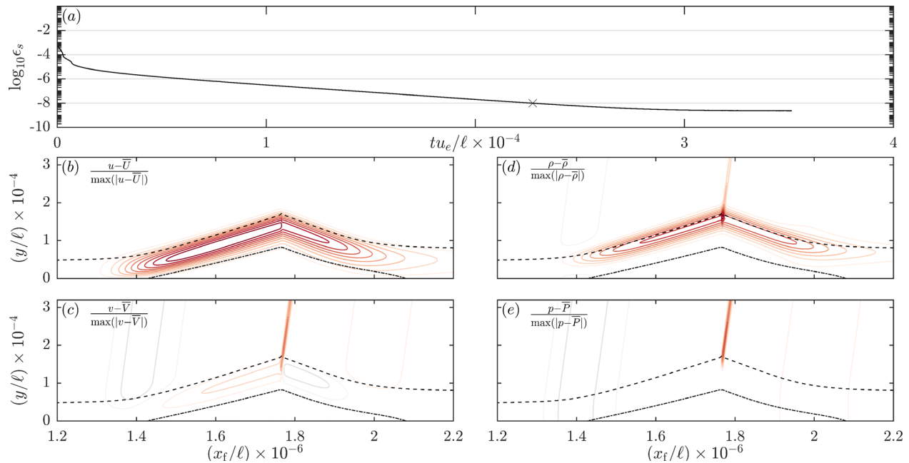
FIG. 2. (a) SFD residual \epsilon_s = \|\mathbf{q} - \mathbf{q}_f\|_{L_2}/\sqrt{S} as a function of the physical time. Perturbation shape in space when \epsilon_s = 10^{-8} [indicated by \times in (a)]: (b) (u - \bar{U})/\max(|u - \bar{U}|) ; (c) (v - \bar{V})/\max(|v - \bar{V}|) ; (d) (\rho - \bar{P})/\max(|\rho - \bar{P}|) ; and (e) (p - \bar{P})/\max(|p - \bar{P}|) [colored lines, 20 contours from minimum (−1, gray) to maximum (1, red)]. (b)–(e) Boundary-layer edge ( \delta_{90} , dashed); \bar{U} = 0 (dash-dotted).
