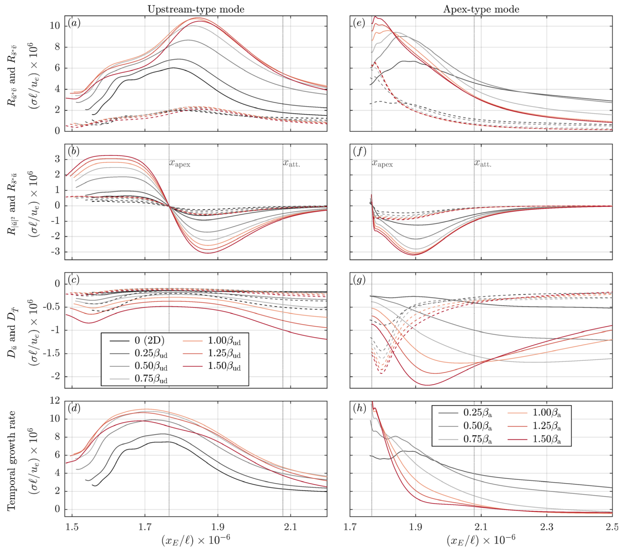
FIG. 8. Streamwise variation of the dominant contributions to the temporal growth rate [Eq. (26)] of the temporal wave packets: (a) and (e) R_{\tilde{u}^* \tilde{v}} (solid) and R_{\tilde{s}^* \tilde{v}} (dashed), (b) and (f) R_{|\tilde{u}|^2} (solid) and R_{\tilde{s}^* \tilde{u}} (dashed), (c) and (g) D_{\tilde{u}} (solid) and D_{\tilde{T}} (dashed), and (d) and (h) temporal growth rate \sigma(t) . (a)–(d) Upstream- and (e)–(h) apex-type modes for relevant \beta -values. (a)–(h) Vertical dotted lines: streamwise location of the bubble apex and reattachment.
