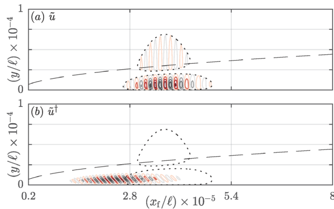
FIG. 10. (a) and (b) Isocontour of |\tilde{u}|/|\tilde{u}|_{\max} (dotted black, level: 1/9) and isocontours [colored lines, from minimum (gray) to maximum (red) with \Delta = 2/9 ] of (a) \mathcal{R}\{\tilde{u}\}/|\tilde{u}|_{\max} and (b) \mathcal{R}\{\tilde{u}^\dagger\}/|\tilde{u}^\dagger|_{\max} corresponding to the most unstable eigenfunction at c_f/u_e = 0.415 . \tilde{U} = 0.9u_e -isocontour (dashed black).
