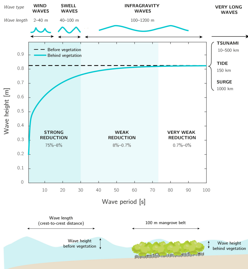
Figure 3. Diagram illustrating the amount of wave reduction for a fixed value of incoming wave height and varying wave periods through a 100 m-wide mangrove belt. The diagram was derived using the model of Mendez and Losada [28] with mangrove vegetation parameters obtained from Suzuki [29]; vegetation density of 1.1 trees/m 2 and tree diameter of 0.27 m. The results were obtained with a water depth of 1.5 m and a wave height of 0.8 m (maximum wave height possible with a breaking ratio of 0.55). The wave lengths indicated in the figure were also calculated for a water depth of 1.5 m.
