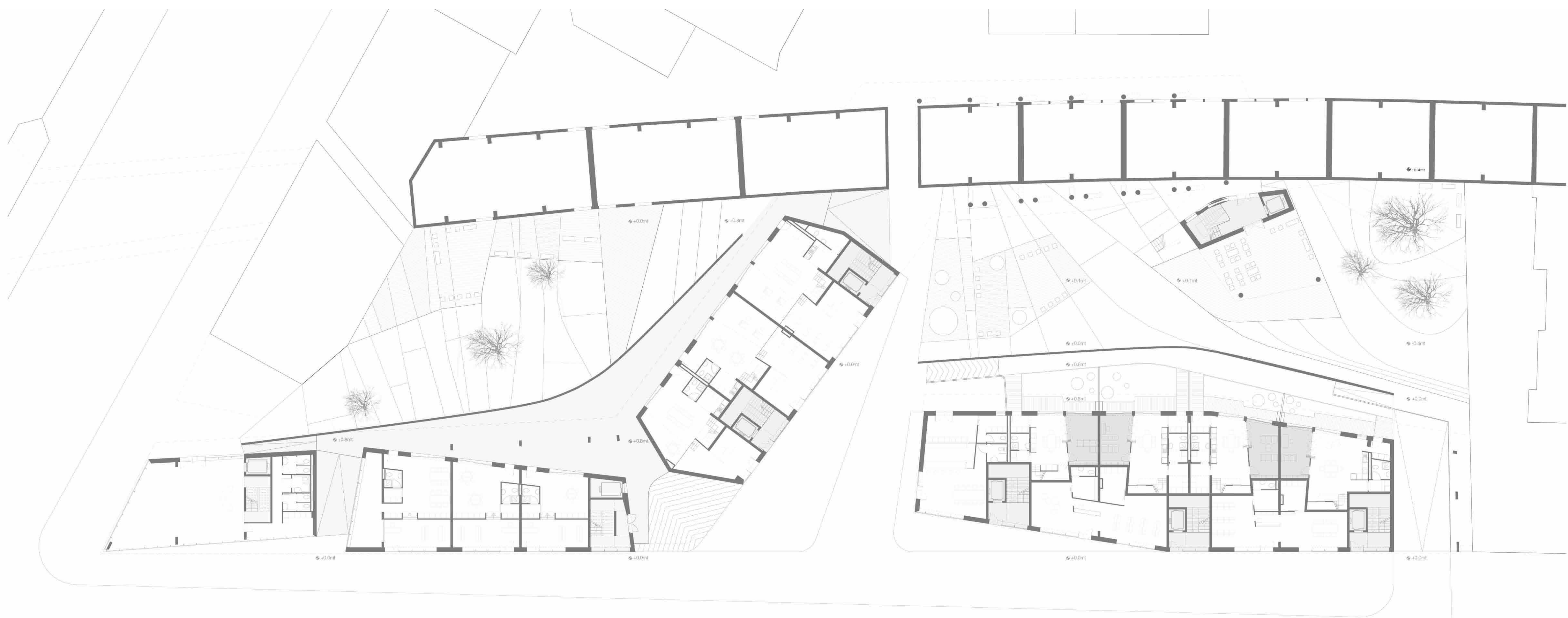
GROUND FLOOR | scale 1:200
