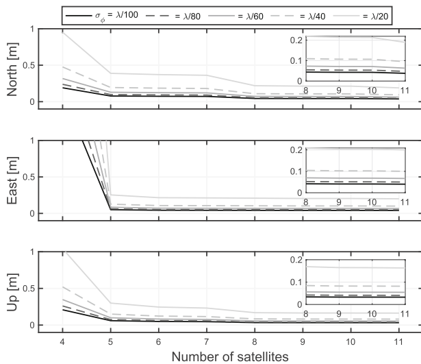
Fig. 9 RMSs (m) of ambiguity-float positioning solutions (left), and the corresponding float-to-fixed RMS ratios and fixed-to-all ambiguity number ratios (%) after partial IAR with a minimum required ILS success-rate of 99.9% (right) as a function of the number of Iridium satellites m for different carrier phase measurement precision \sigma_\phi , based on the dual-epoch phase-only model (14) with a 30-s sampling interval
